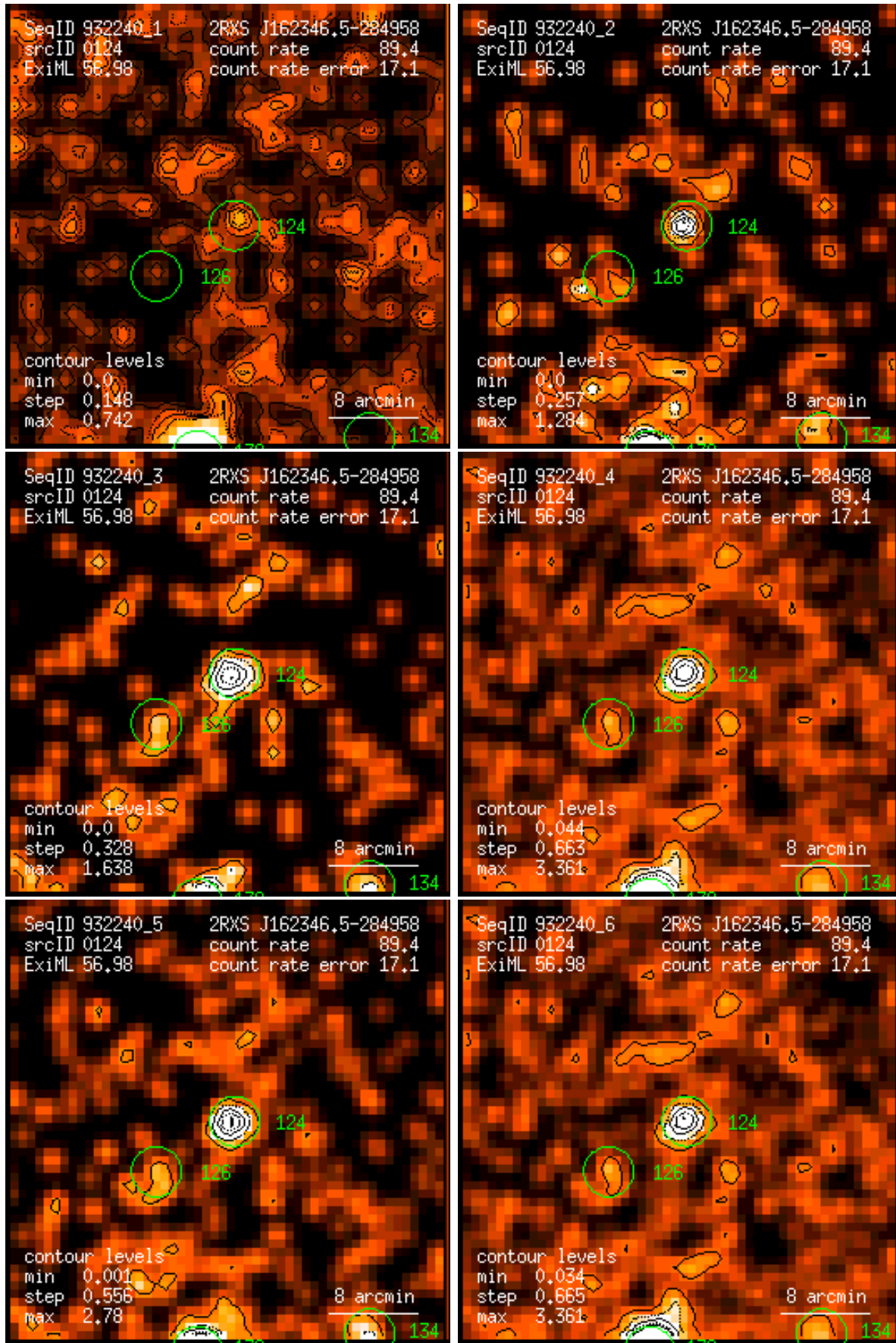
Figure 124: RASS 932240: detection 0124: band rate images, Gaussian filter: (1) PSPC channels 11 – 41, (2) 52 – 90, (3) 91 – 201, (4) 11 – 235, (5) 52 – 201, (6) 11 – 201. Broad band rates in counts/ks. Band rate contour levels in counts/ks/arcmin 2 .
