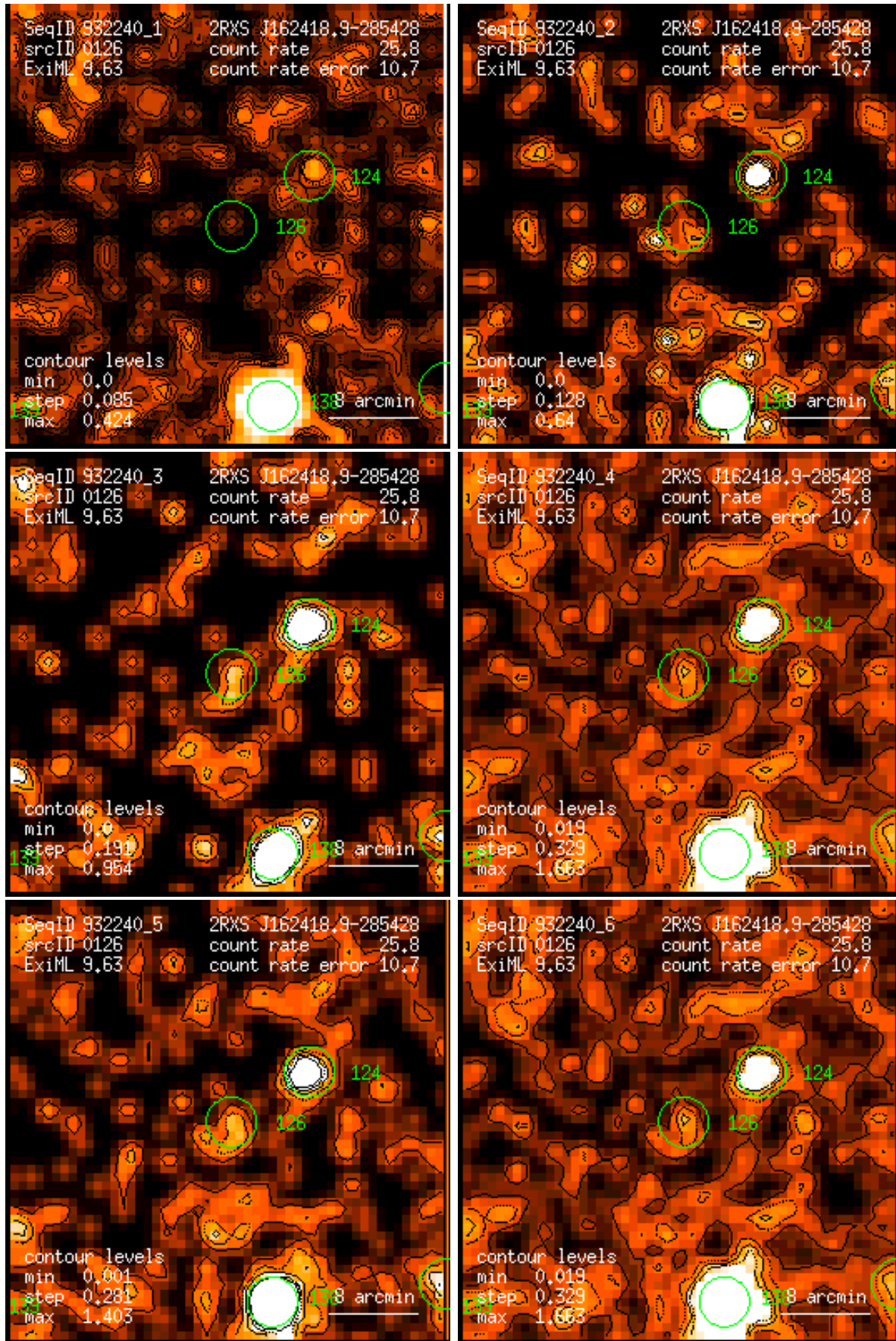
Figure 126: RASS 932240: detection 0126: band rate images, Gaussian filter: (1) PSPC channels 11 – 41, (2) 52 – 90, (3) 91 – 201, (4) 11 – 235, (5) 52 – 201, (6) 11 – 201. Broad band rates in counts/ks. Band rate contour levels in counts/ks/arcmin 2 .
