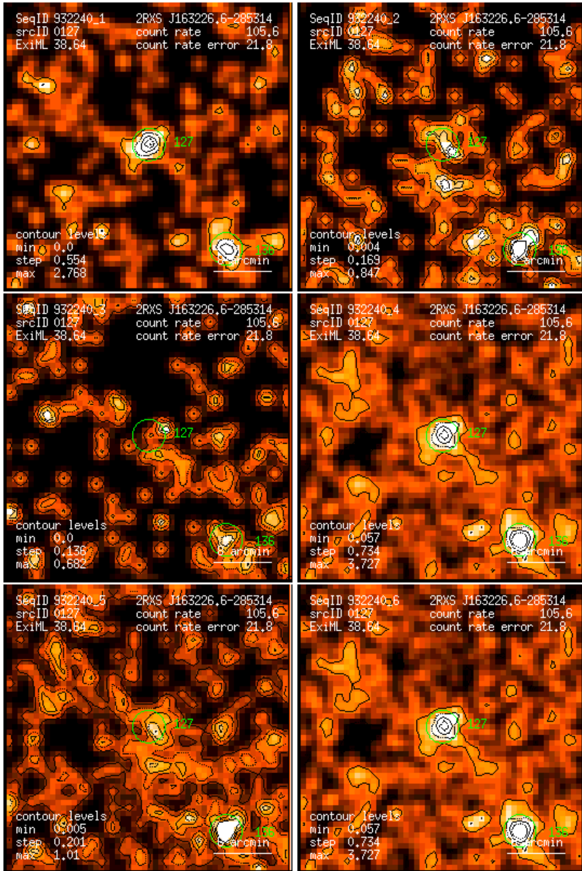
Figure 127: RASS 932240: detection 0127: band rate images, Gaussian filter: (1) PSPC channels 11 – 41, (2) 52 – 90, (3) 91 – 201, (4) 11 – 235, (5) 52 – 201, (6) 11 – 201. Broad band rates in counts/ks. Band rate contour levels in counts/ks/arcmin 2 .
