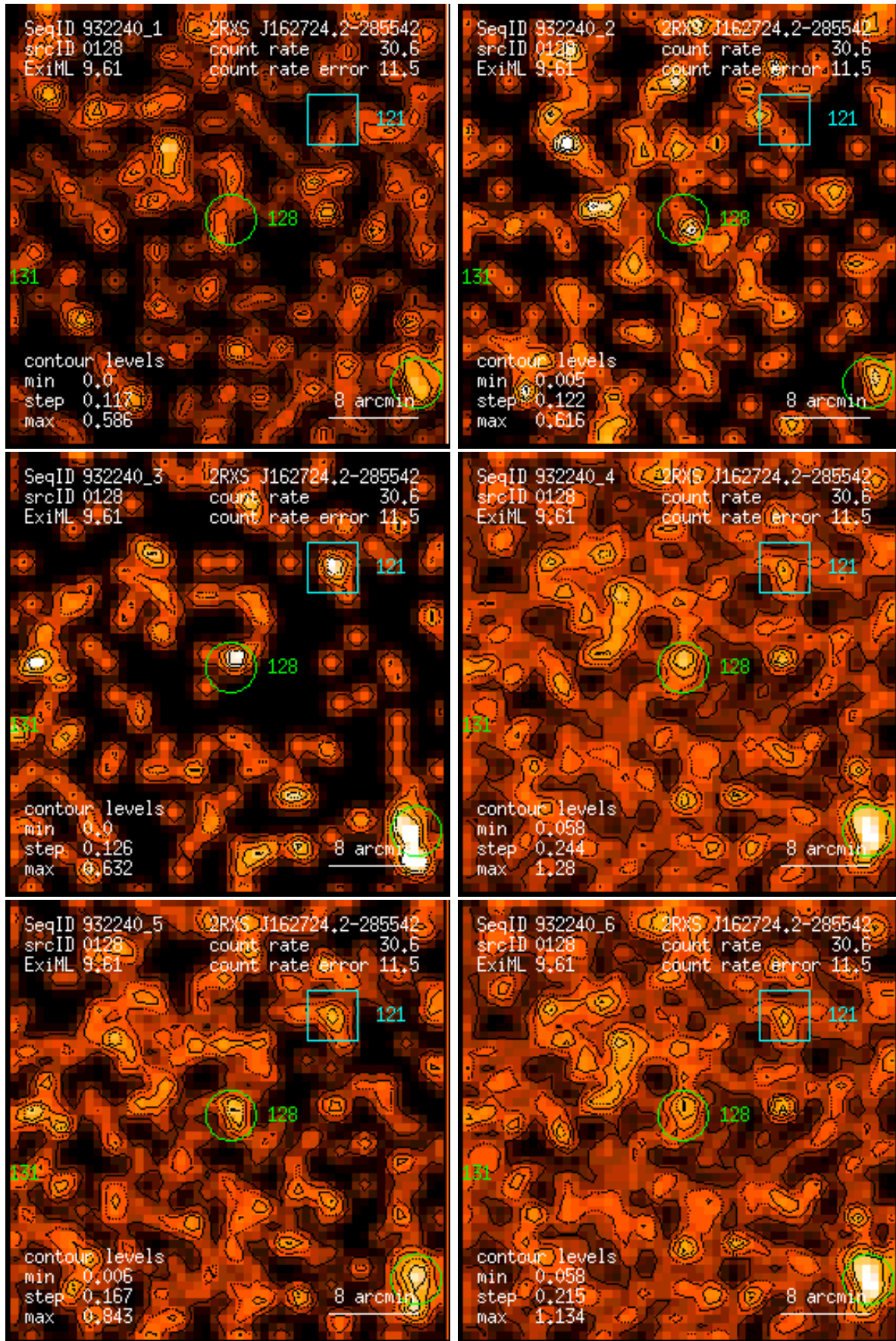
Figure 128: RASS 932240: detection 0128: band rate images, Gaussian filter: (1) PSPC channels 11 – 41, (2) 52 – 90, (3) 91 – 201, (4) 11 – 235, (5) 52 – 201, (6) 11 – 201. Broad band rates in counts/ks. Band rate contour levels in counts/ks/arcmin 2 .
