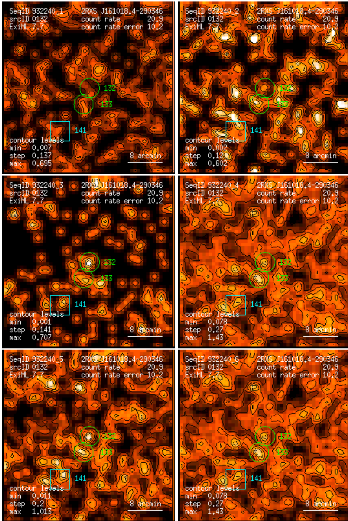
Figure 132: RASS 932240: detection 0132: band rate images, Gaussian filter: (1) PSPC channels 11 – 41, (2) 52 – 90, (3) 91 – 201, (4) 11 – 235, (5) 52 – 201, (6) 11 – 201. Broad band rates in counts/ks. Band rate contour levels in counts/ks/arcmin 2 .
