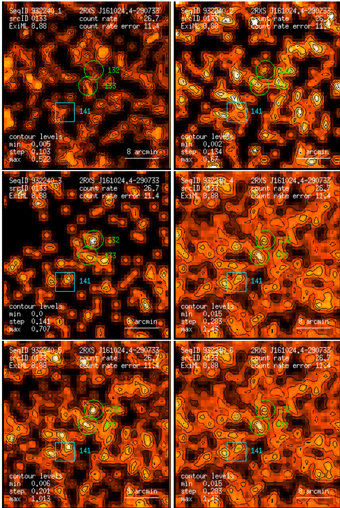
Figure 133: RASS 932240: detection 0133: band rate images, Gaussian filter: (1) PSPC channels 11 – 41, (2) 52 – 90, (3) 91 – 201, (4) 11 – 235, (5) 52 – 201, (6) 11 – 201. Broad band rates in counts/ks. Band rate contour levels in counts/ks/arcmin 2 .
