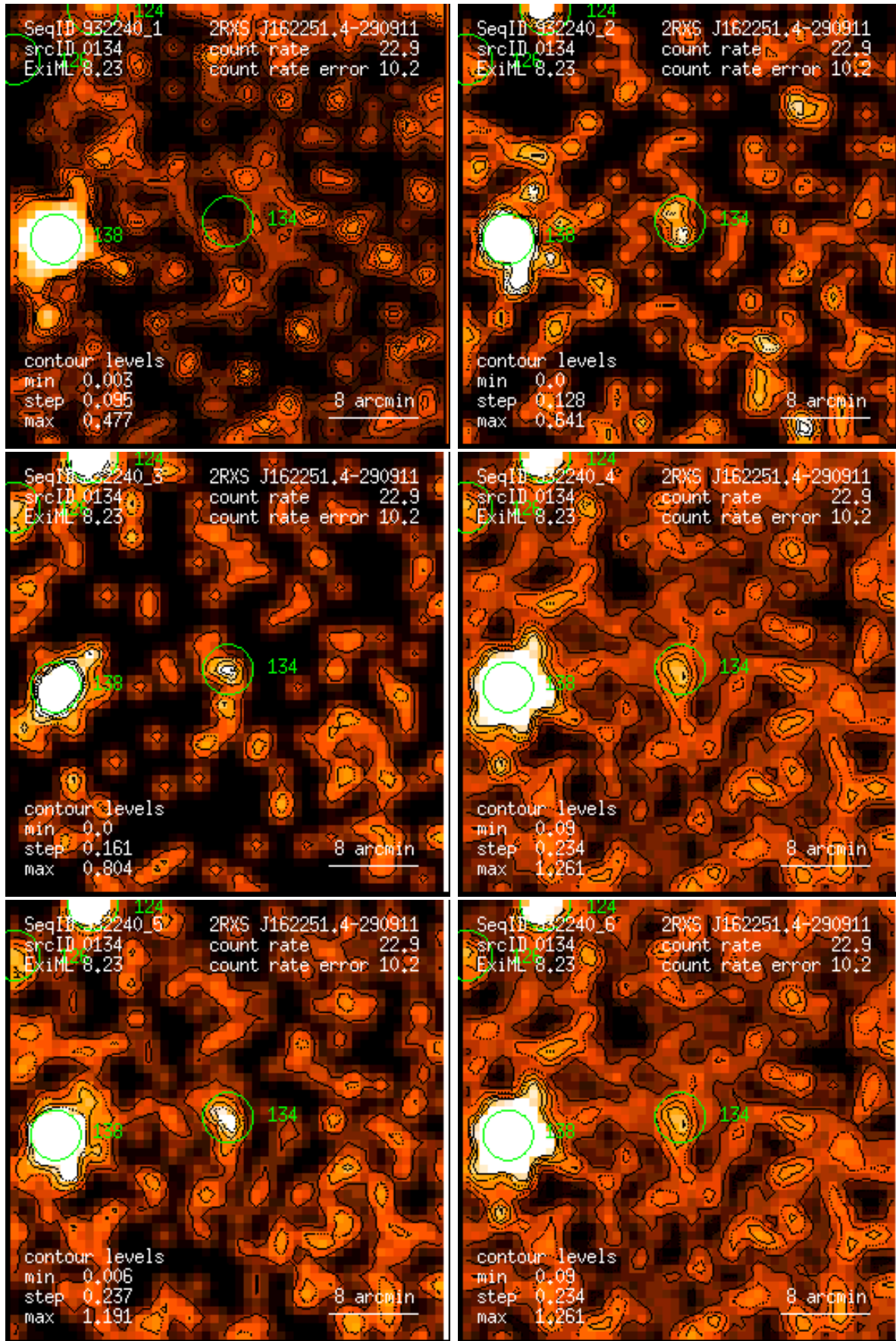
Figure 134: RASS 932240: detection 0134: band rate images, Gaussian filter: (1) PSPC channels 11 – 41, (2) 52 – 90, (3) 91 – 201, (4) 11 – 235, (5) 52 – 201, (6) 11 – 201. Broad band rates in counts/ks. Band rate contour levels in counts/ks/arcmin 2 .
