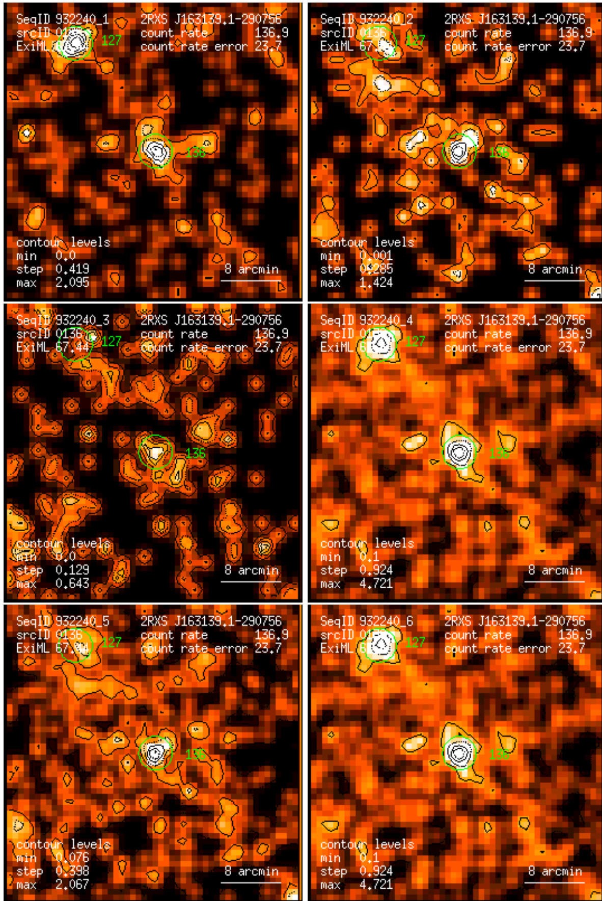
Figure 136: RASS 932240: detection 0136: band rate images, Gaussian filter: (1) PSPC channels 11 – 41, (2) 52 – 90, (3) 91 – 201, (4) 11 – 235, (5) 52 – 201, (6) 11 – 201. Broad band rates in counts/ks. Band rate contour levels in counts/ks/arcmin 2 .
