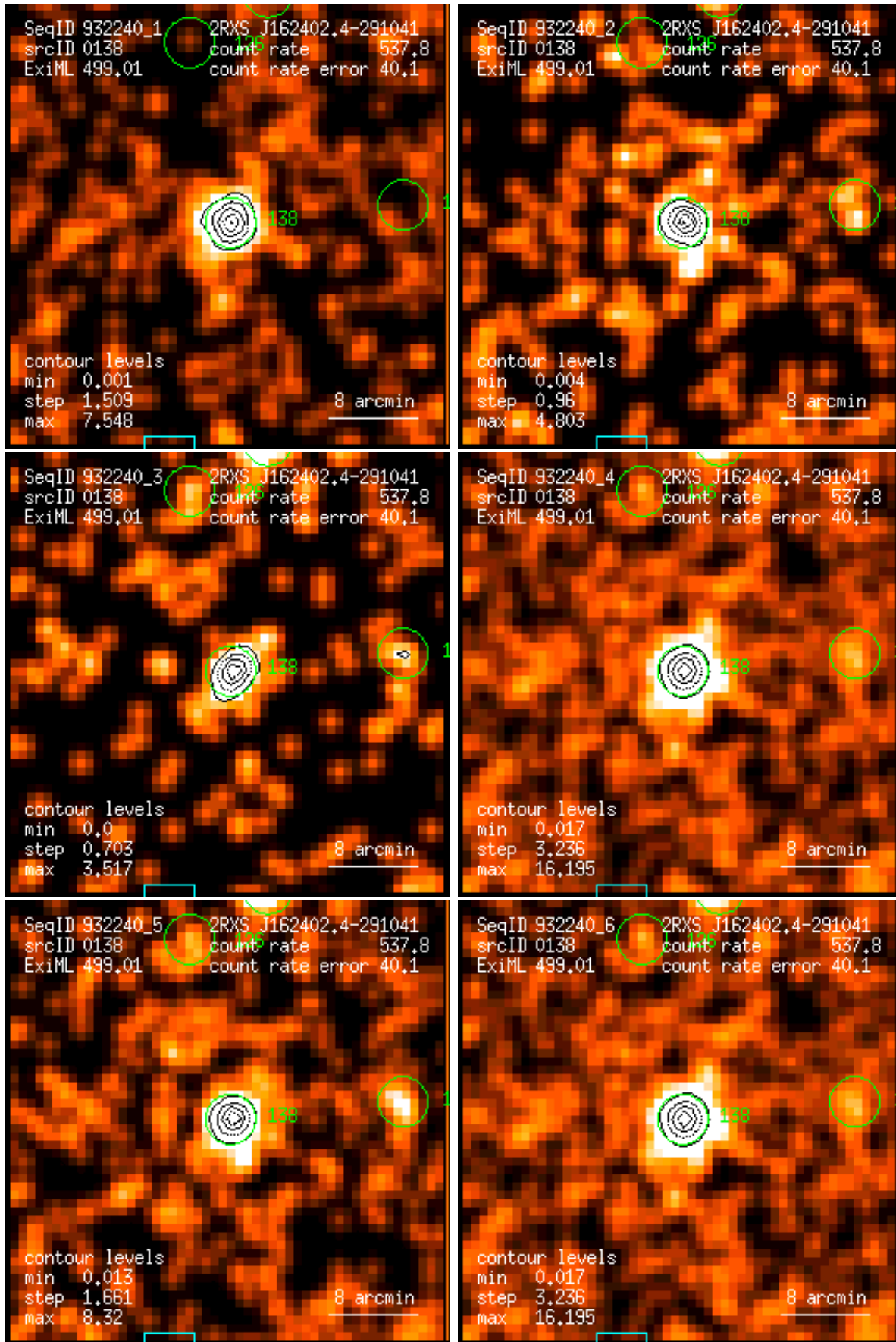
Figure 138: RASS 932240: detection 0138: band rate images, Gaussian filter: (1) PSPC channels 11 – 41, (2) 52 – 90, (3) 91 – 201, (4) 11 – 235, (5) 52 – 201, (6) 11 – 201. Broad band rates in counts/ks. Band rate contour levels in counts/ks/arcmin 2 .
