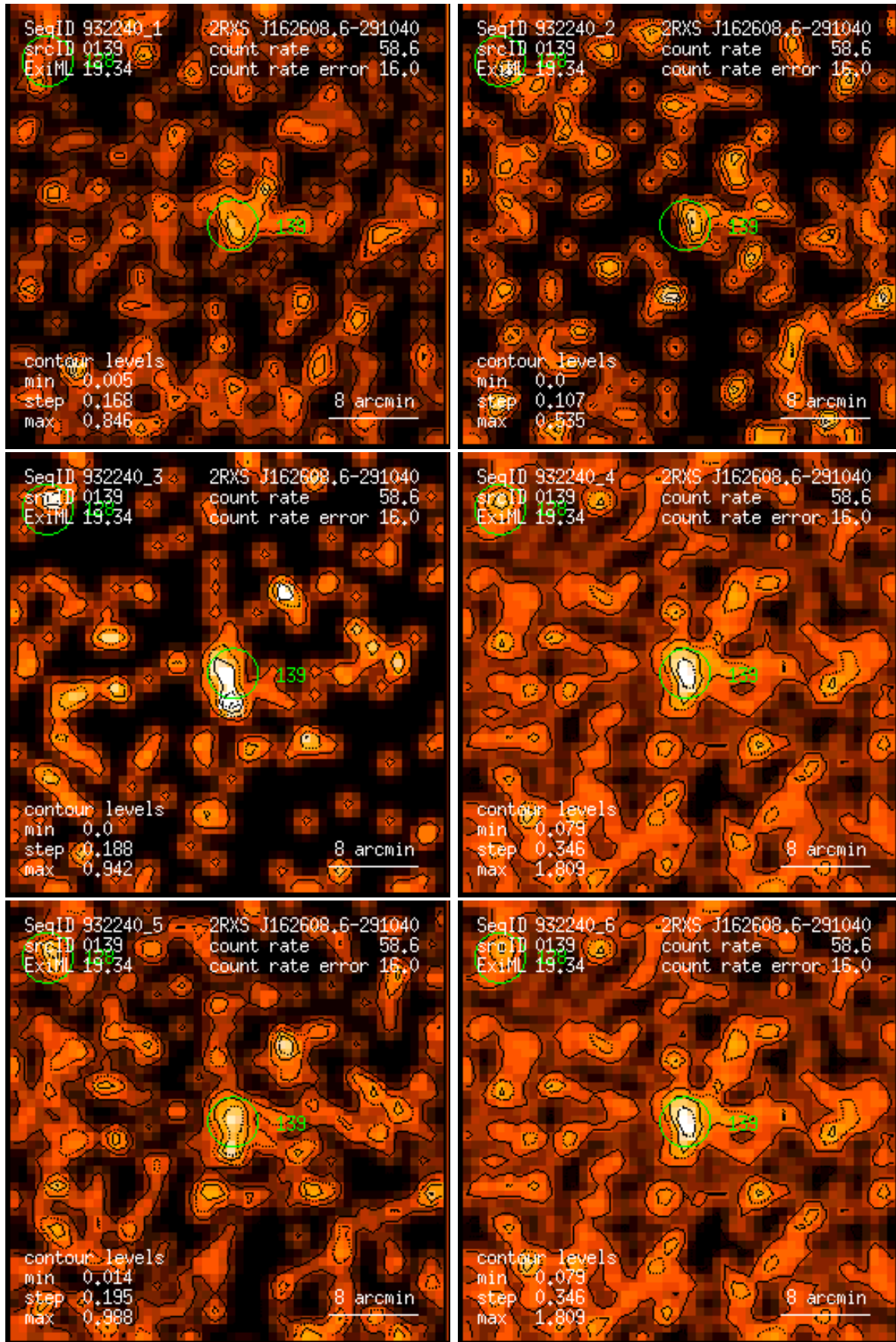
Figure 139: RASS 932240: detection 0139: band rate images, Gaussian filter: (1) PSPC channels 11 – 41, (2) 52 – 90, (3) 91 – 201, (4) 11 – 235, (5) 52 – 201, (6) 11 – 201. Broad band rates in counts/ks. Band rate contour levels in counts/ks/arcmin 2 .
