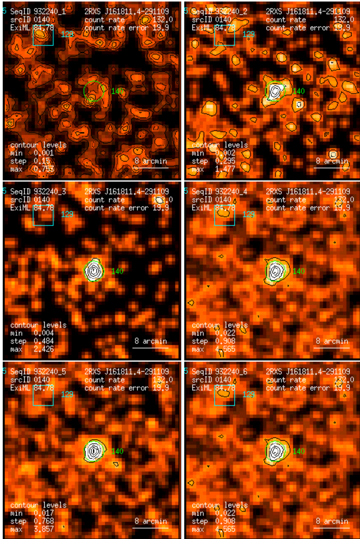
Figure 140: RASS 932240: detection 0140: band rate images, Gaussian filter: (1) PSPC channels 11 – 41, (2) 52 – 90, (3) 91 – 201, (4) 11 – 235, (5) 52 – 201, (6) 11 – 201. Broad band rates in counts/ks. Band rate contour levels in counts/ks/arcmin 2 .
