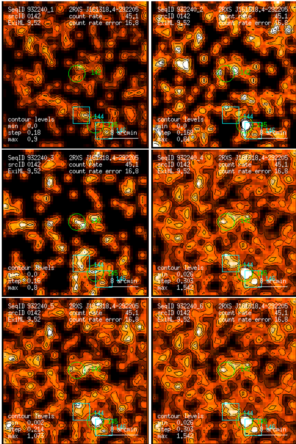
Figure 142: RASS 932240: detection 0142: band rate images, Gaussian filter: (1) PSPC channels 11 – 41, (2) 52 – 90, (3) 91 – 201, (4) 11 – 235, (5) 52 – 201, (6) 11 – 201. Broad band rates in counts/ks. Band rate contour levels in counts/ks/arcmin 2 .
