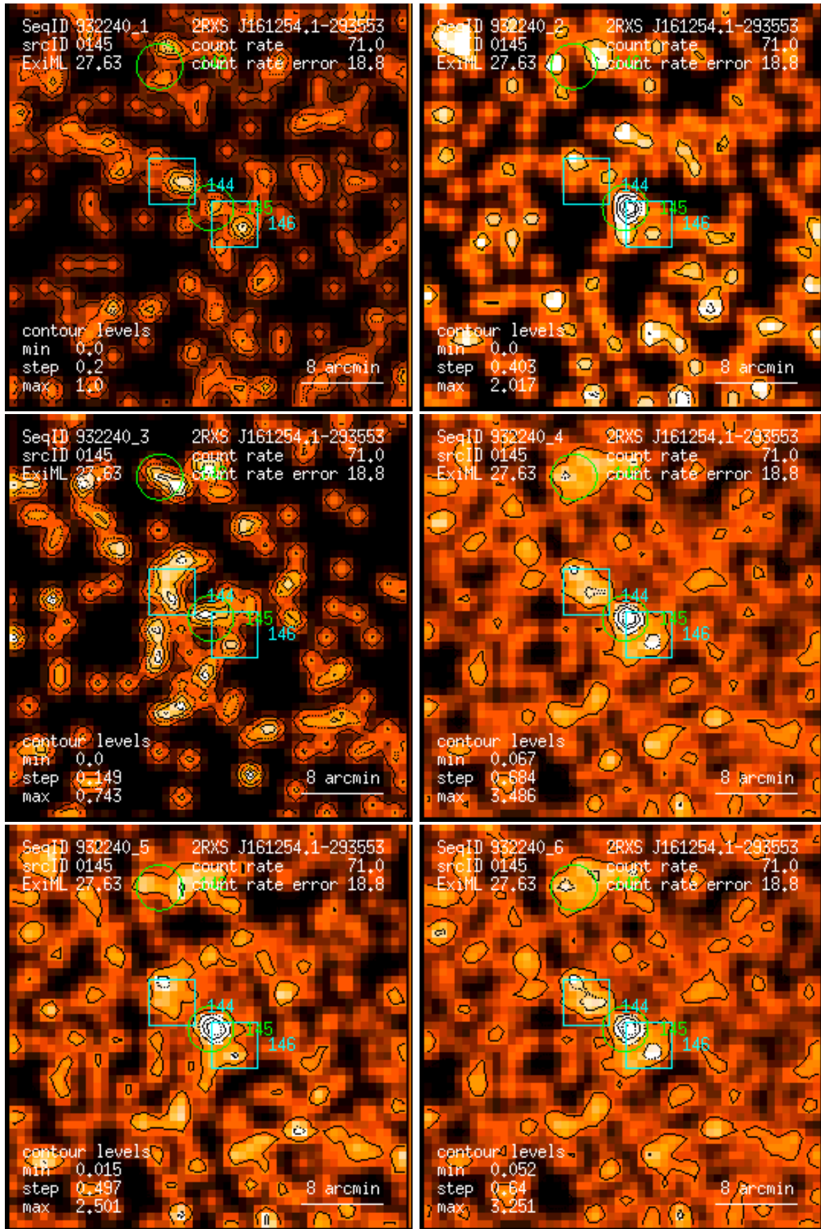
Figure 145: RASS 932240: detection 0145: band rate images, Gaussian filter: (1) PSPC channels 11 – 41, (2) 52 – 90, (3) 91 – 201, (4) 11 – 235, (5) 52 – 201, (6) 11 – 201. Broad band rates in counts/ks. Band rate contour levels in counts/ks/arcmin 2 .
