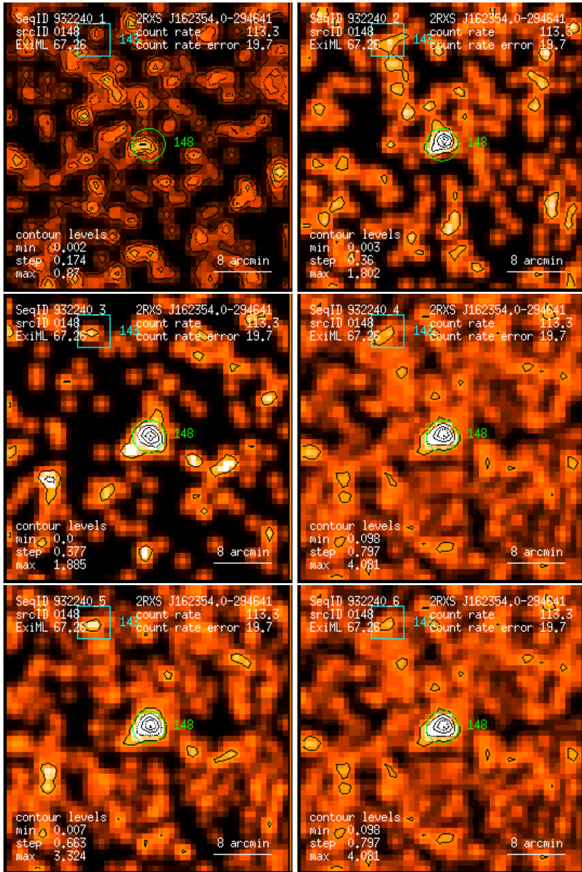
Figure 148: RASS 932240: detection 0148: band rate images, Gaussian filter: (1) PSPC channels 11 – 41, (2) 52 – 90, (3) 91 – 201, (4) 11 – 235, (5) 52 – 201, (6) 11 – 201. Broad band rates in counts/ks. Band rate contour levels in counts/ks/arcmin 2 .
