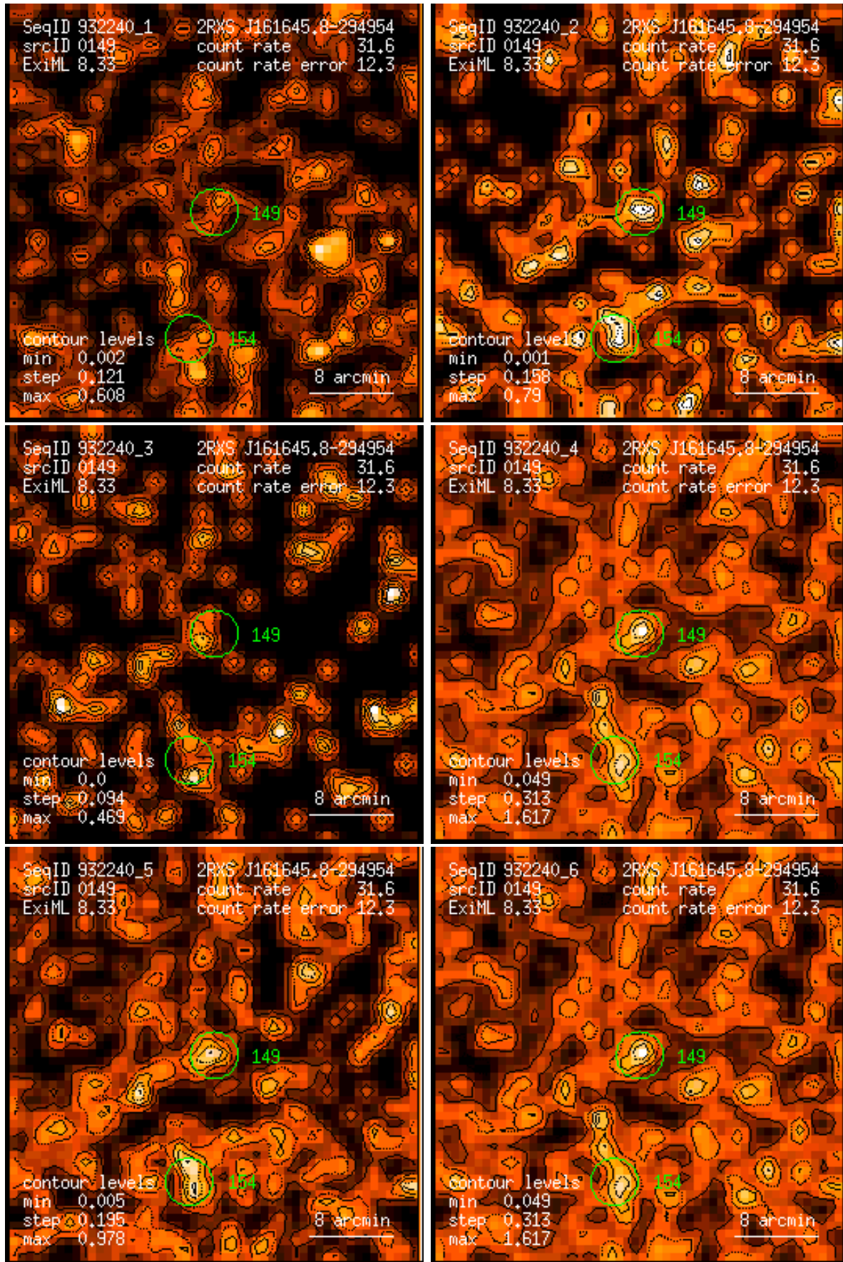
Figure 149: RASS 932240: detection 0149: band rate images, Gaussian filter: (1) PSPC channels 11 – 41, (2) 52 – 90, (3) 91 – 201, (4) 11 – 235, (5) 52 – 201, (6) 11 – 201. Broad band rates in counts/ks. Band rate contour levels in counts/ks/arcmin 2 .
