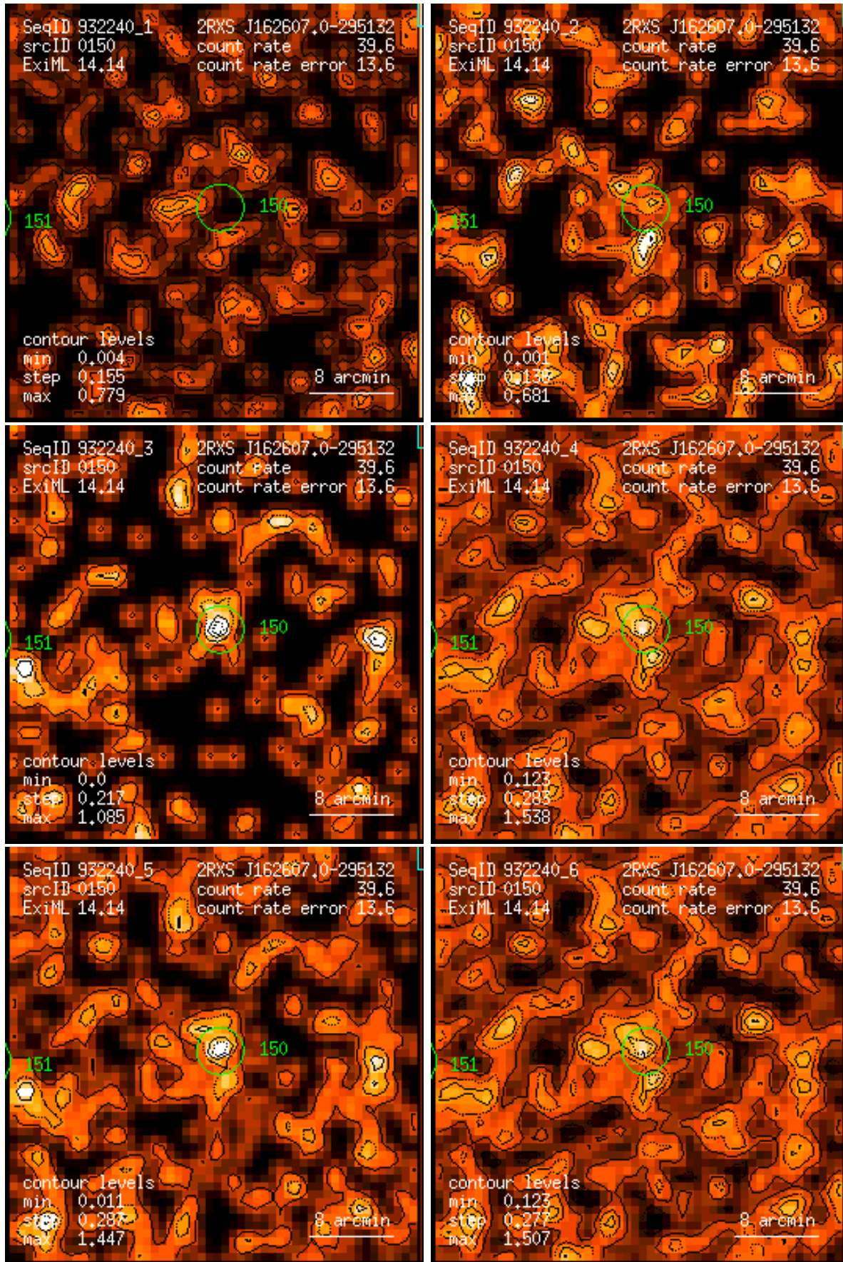
Figure 150: RASS 932240: detection 0150: band rate images, Gaussian filter: (1) PSPC channels 11 – 41, (2) 52 – 90, (3) 91 – 201, (4) 11 – 235, (5) 52 – 201, (6) 11 – 201. Broad band rates in counts/ks. Band rate contour levels in counts/ks/arcmin 2 .
