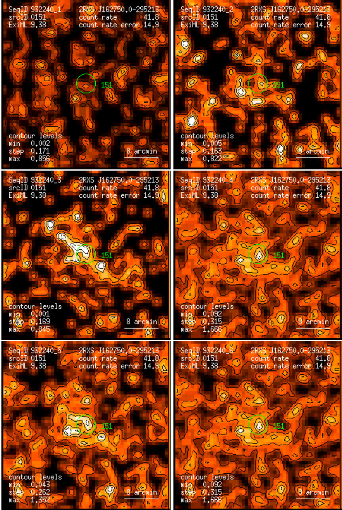
Figure 151: RASS 932240: detection 0151: band rate images, Gaussian filter: (1) PSPC channels 11 – 41, (2) 52 – 90, (3) 91 – 201, (4) 11 – 235, (5) 52 – 201, (6) 11 – 201. Broad band rates in counts/ks. Band rate contour levels in counts/ks/arcmin 2 .
