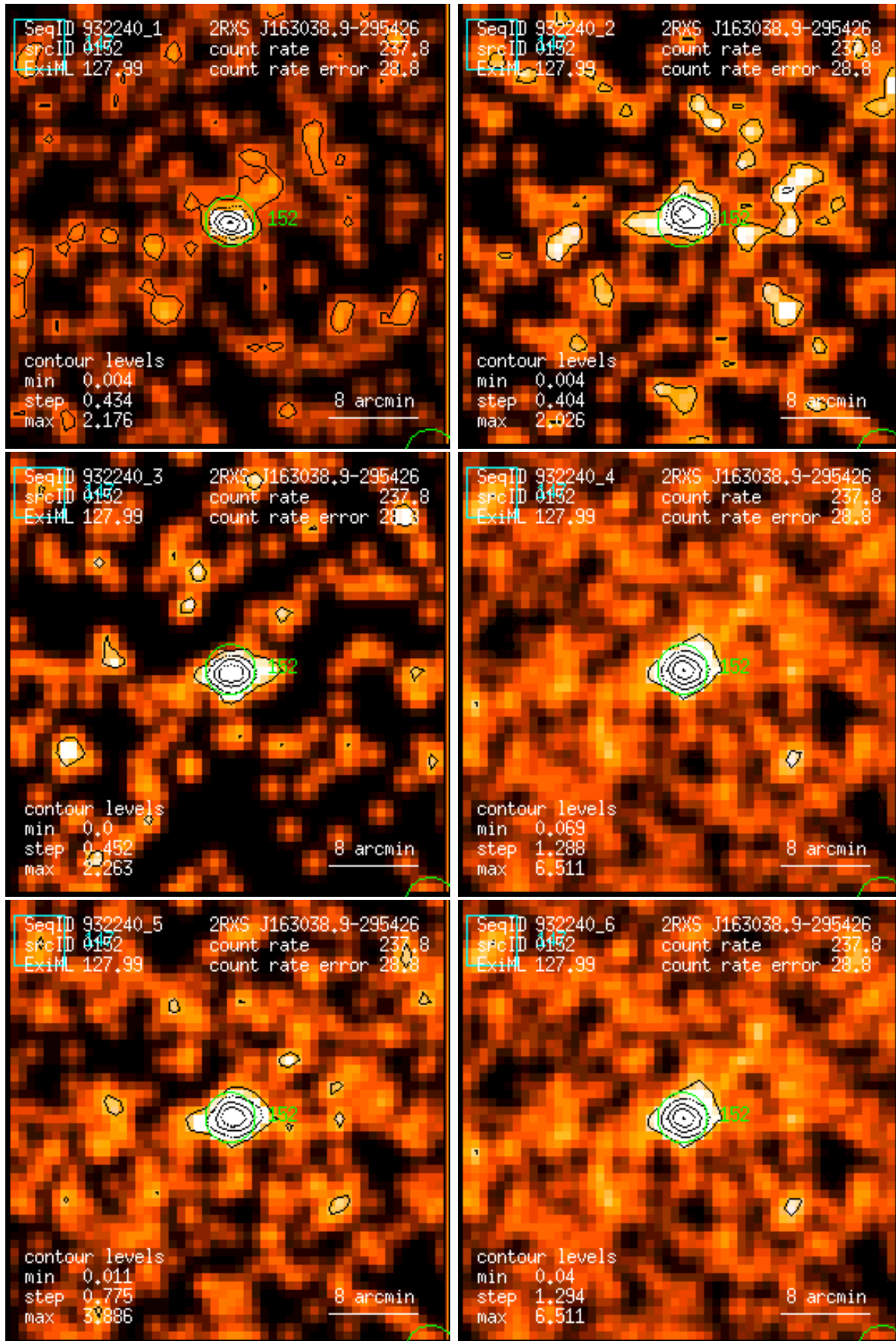
Figure 152: RASS 932240: detection 0152: band rate images, Gaussian filter: (1) PSPC channels 11 – 41, (2) 52 – 90, (3) 91 – 201, (4) 11 – 235, (5) 52 – 201, (6) 11 – 201. Broad band rates in counts/ks. Band rate contour levels in counts/ks/arcmin 2 .
