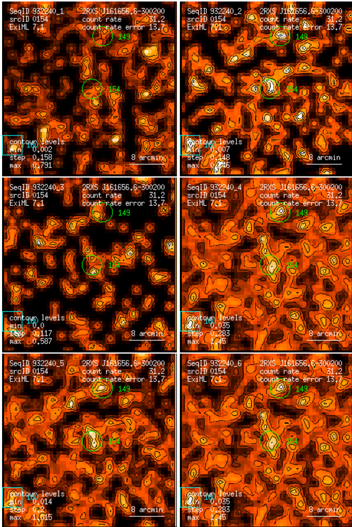
Figure 154: RASS 932240: detection 0154: band rate images, Gaussian filter: (1) PSPC channels 11 – 41, (2) 52 – 90, (3) 91 – 201, (4) 11 – 235, (5) 52 – 201, (6) 11 – 201. Broad band rates in counts/ks. Band rate contour levels in counts/ks/arcmin 2 .
