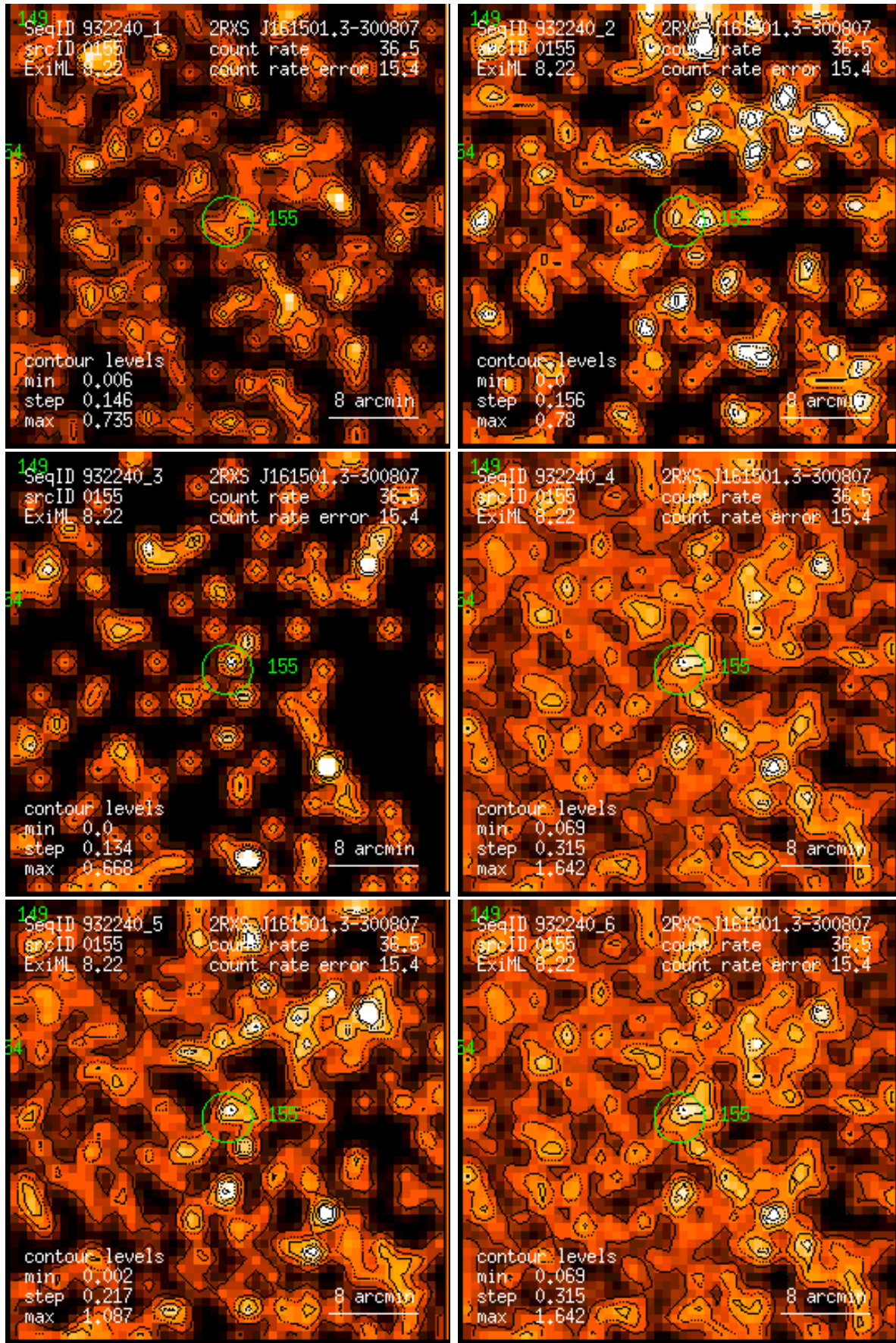
Figure 155: RASS 932240: detection 0155: band rate images, Gaussian filter: (1) PSPC channels 11 – 41, (2) 52 – 90, (3) 91 – 201, (4) 11 – 235, (5) 52 – 201, (6) 11 – 201. Broad band rates in counts/ks. Band rate contour levels in counts/ks/arcmin 2 .
