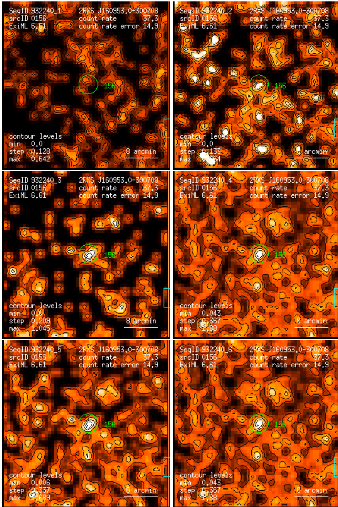
Figure 156: RASS 932240: detection 0156: band rate images, Gaussian filter: (1) PSPC channels 11 – 41, (2) 52 – 90, (3) 91 – 201, (4) 11 – 235, (5) 52 – 201, (6) 11 – 201. Broad band rates in counts/ks. Band rate contour levels in counts/ks/arcmin 2 .
