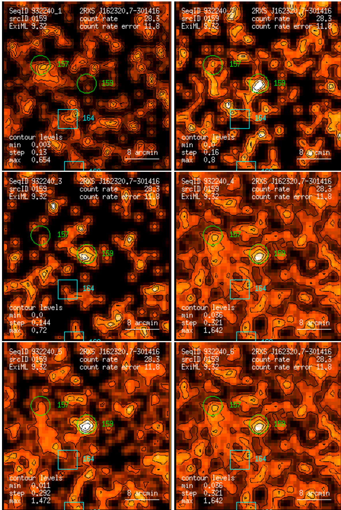
Figure 159: RASS 932240: detection 0159: band rate images, Gaussian filter: (1) PSPC channels 11 – 41, (2) 52 – 90, (3) 91 – 201, (4) 11 – 235, (5) 52 – 201, (6) 11 – 201. Broad band rates in counts/ks. Band rate contour levels in counts/ks/arcmin 2 .
