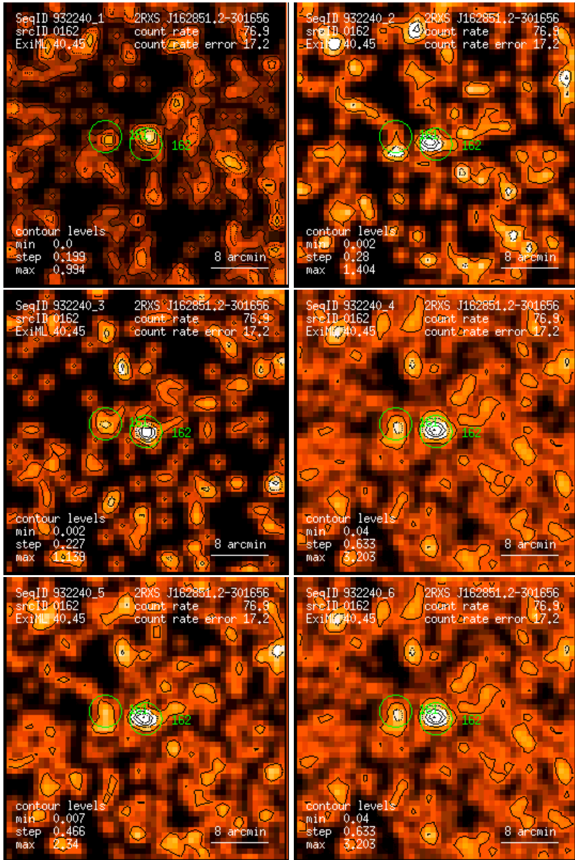
Figure 162: RASS 932240: detection 0162: band rate images, Gaussian filter: (1) PSPC channels 11 – 41, (2) 52 – 90, (3) 91 – 201, (4) 11 – 235, (5) 52 – 201, (6) 11 – 201. Broad band rates in counts/ks. Band rate contour levels in counts/ks/arcmin 2 .
