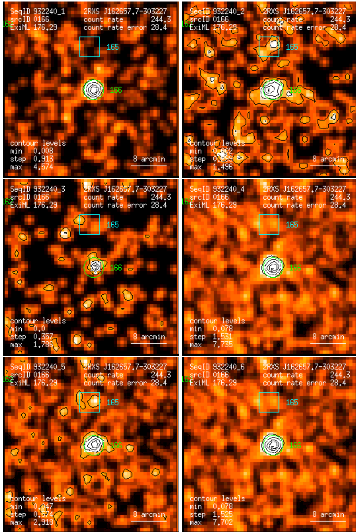
Figure 166: RASS 932240: detection 0166: band rate images, Gaussian filter: (1) PSPC channels 11 – 41, (2) 52 – 90, (3) 91 – 201, (4) 11 – 235, (5) 52 – 201, (6) 11 – 201. Broad band rates in counts/ks. Band rate contour levels in counts/ks/arcmin 2 .
