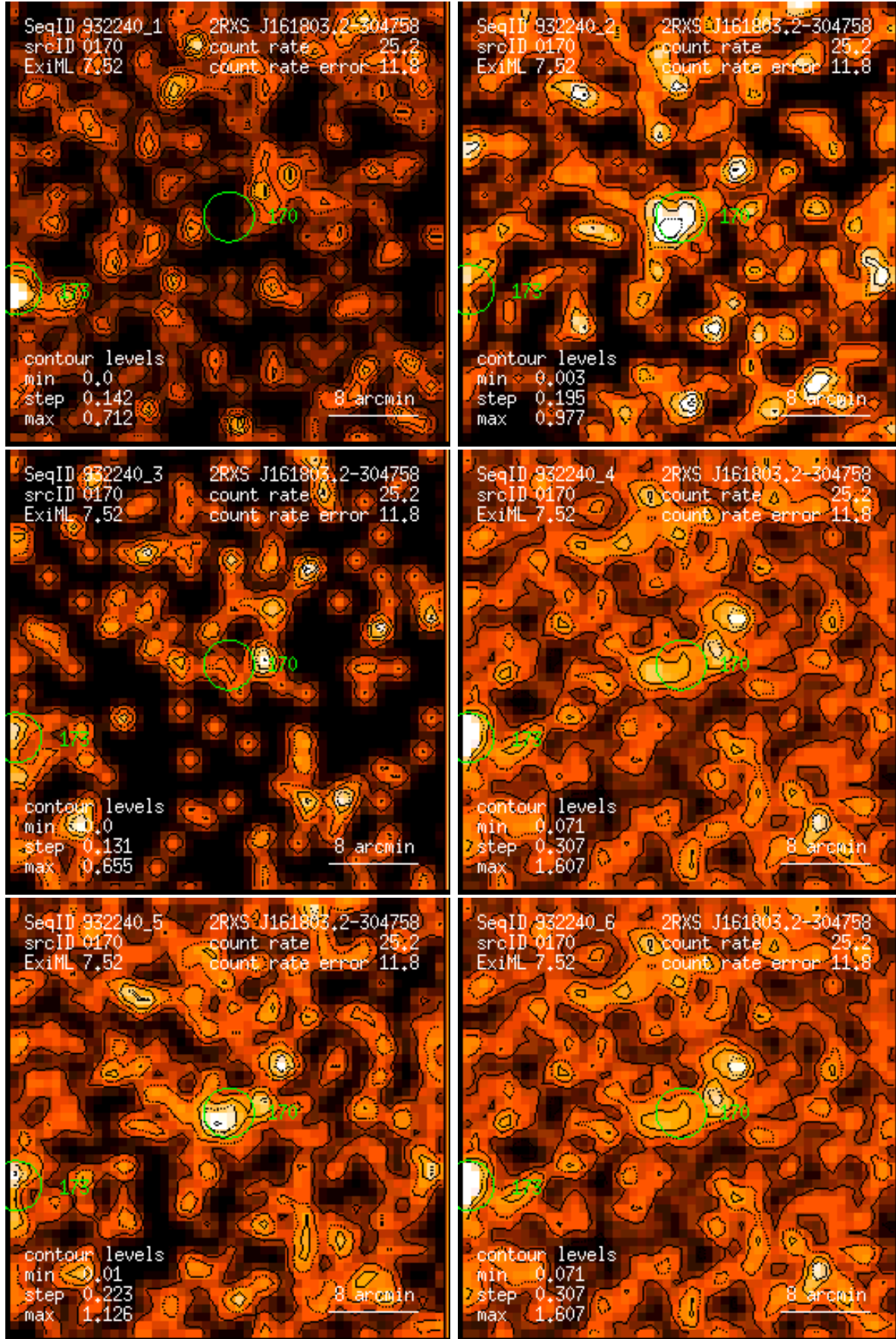
Figure 170: RASS 932240: detection 0170: band rate images, Gaussian filter: (1) PSPC channels 11 – 41, (2) 52 – 90, (3) 91 – 201, (4) 11 – 235, (5) 52 – 201, (6) 11 – 201. Broad band rates in counts/ks. Band rate contour levels in counts/ks/arcmin 2 .
