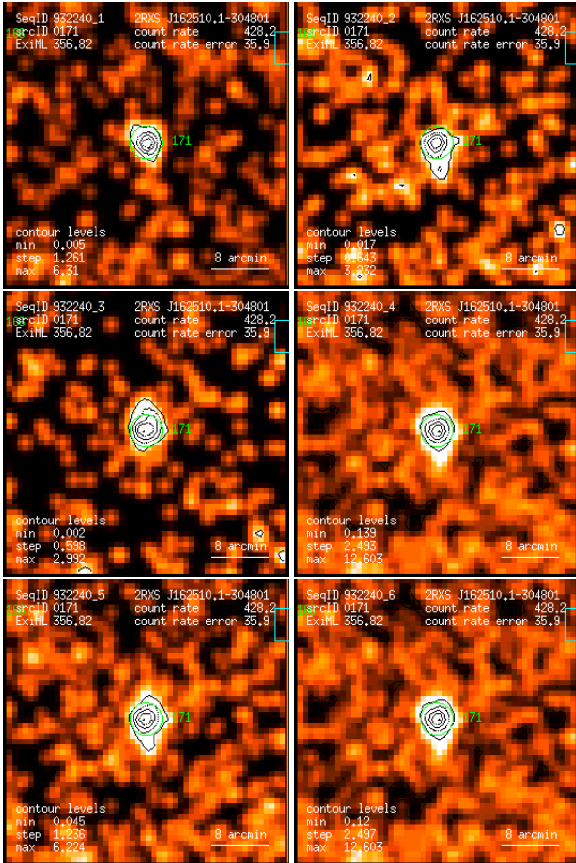
Figure 171: RASS 932240: detection 0171: band rate images, Gaussian filter: (1) PSPC channels 11 – 41, (2) 52 – 90, (3) 91 – 201, (4) 11 – 235, (5) 52 – 201, (6) 11 – 201. Broad band rates in counts/ks. Band rate contour levels in counts/ks/arcmin 2 .
