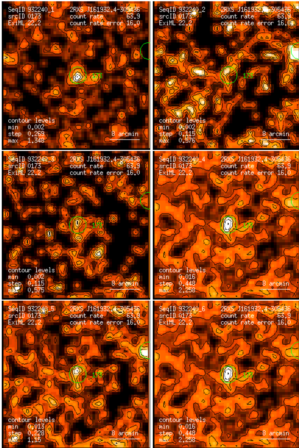
Figure 173: RASS 932240: detection 0173: band rate images, Gaussian filter: (1) PSPC channels 11 – 41, (2) 52 – 90, (3) 91 – 201, (4) 11 – 235, (5) 52 – 201, (6) 11 – 201. Broad band rates in counts/ks. Band rate contour levels in counts/ks/arcmin 2 .
