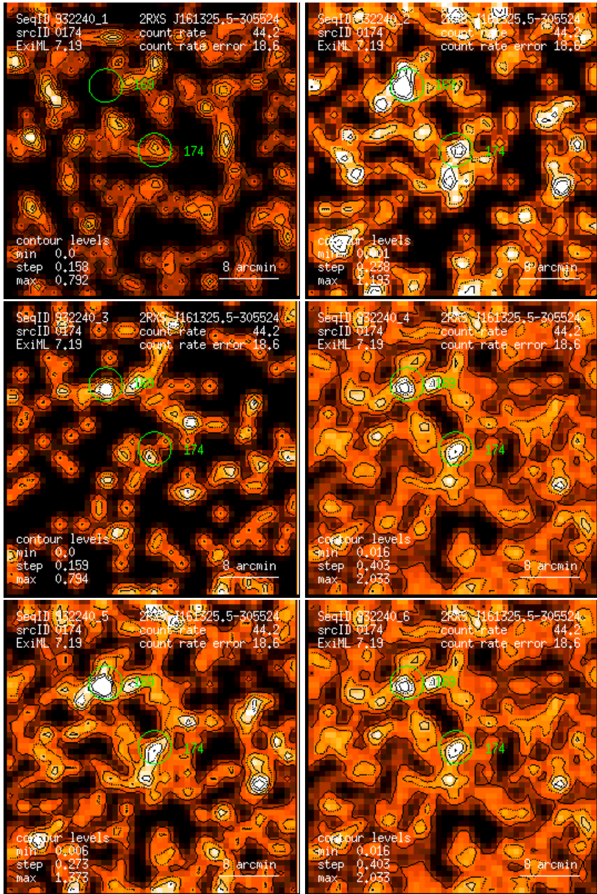
Figure 174: RASS 932240: detection 0174: band rate images, Gaussian filter: (1) PSPC channels 11 – 41, (2) 52 – 90, (3) 91 – 201, (4) 11 – 235, (5) 52 – 201, (6) 11 – 201. Broad band rates in counts/ks. Band rate contour levels in counts/ks/arcmin 2 .
