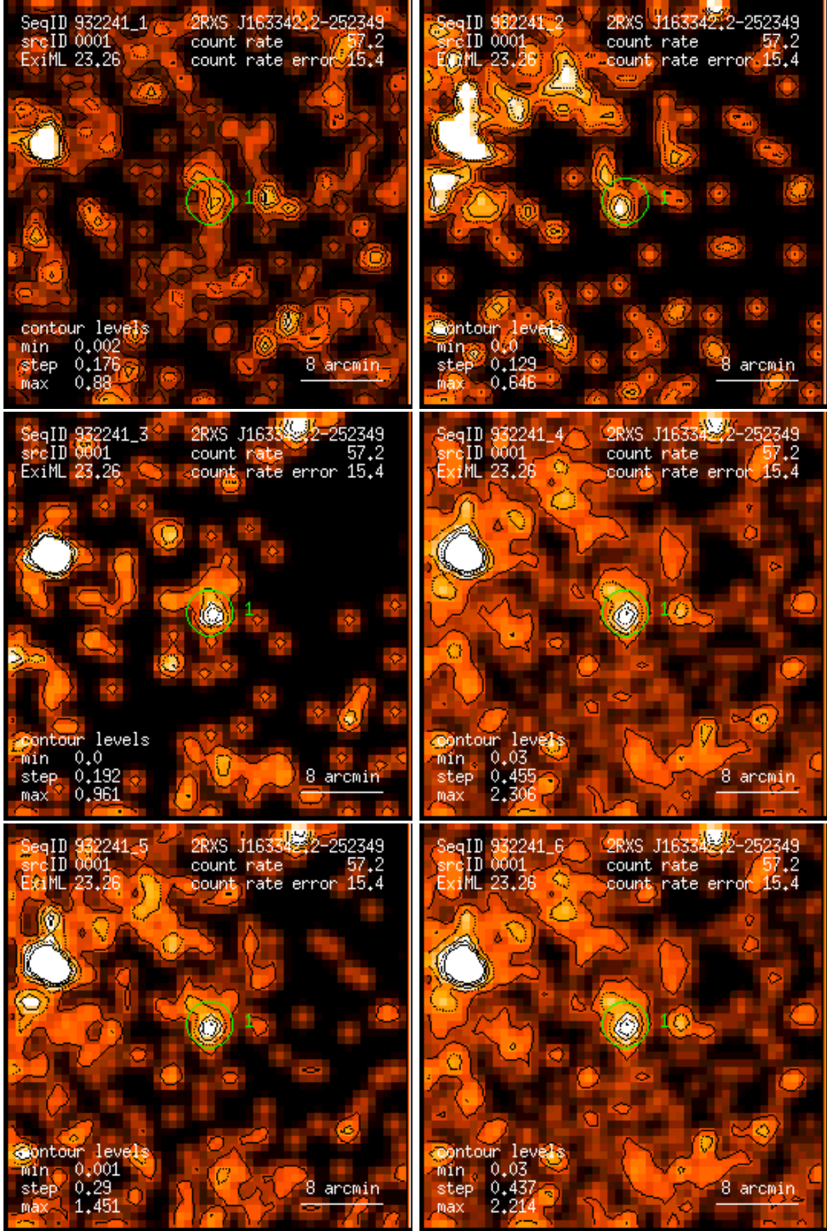
Figure 1: RASS 932241: detection 0001: band rate images, Gaussian filter: (1) PSPC channels 11 – 41, (2) 52 – 90, (3) 91 – 201, (4) 11 – 235, (5) 52 – 201, (6) 11 – 201. Broad band rates in counts/ks. Band rate contour levels in counts/ks/arcmin 2 .
