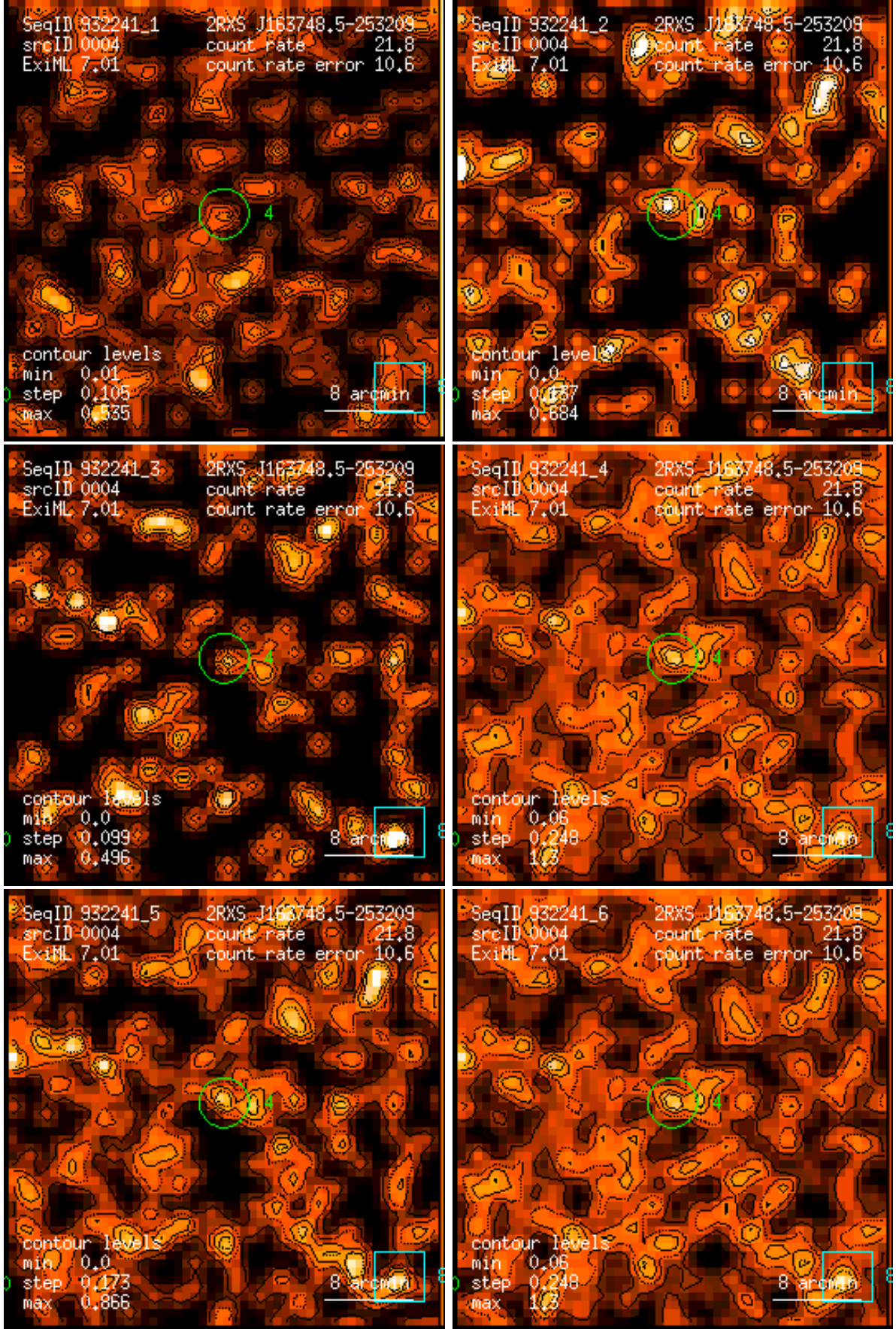
Figure 4: RASS 932241: detection 0004: band rate images, Gaussian filter: (1) PSPC channels 11 – 41, (2) 52 – 90, (3) 91 – 201, (4) 11 – 235, (5) 52 – 201, (6) 11 – 201. Broad band rates in counts/ks. Band rate contour levels in counts/ks/arcmin 2 .
