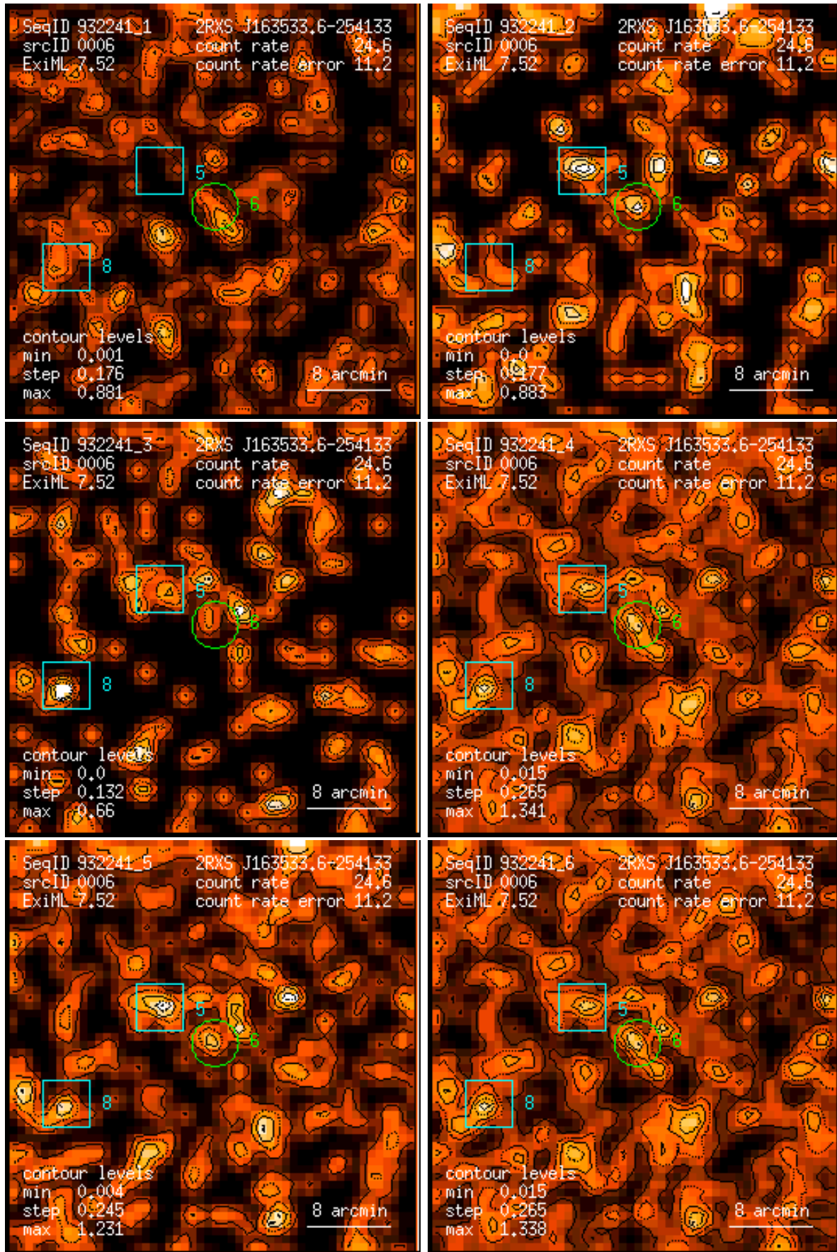
Figure 6: RASS 932241: detection 0006: band rate images, Gaussian filter: (1) PSPC channels 11 – 41, (2) 52 – 90, (3) 91 – 201, (4) 11 – 235, (5) 52 – 201, (6) 11 – 201. Broad band rates in counts/ks. Band rate contour levels in counts/ks/arcmin 2 .
