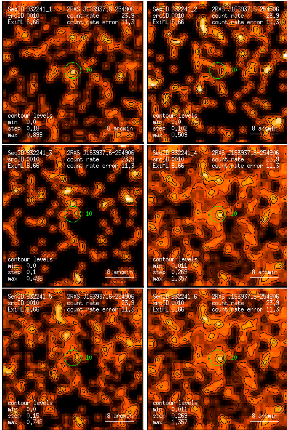
Figure 10: RASS 932241: detection 0010: band rate images, Gaussian filter: (1) PSPC channels 11 – 41, (2) 52 – 90, (3) 91 – 201, (4) 11 – 235, (5) 52 – 201, (6) 11 – 201. Broad band rates in counts/ks. Band rate contour levels in counts/ks/arcmin 2 .
