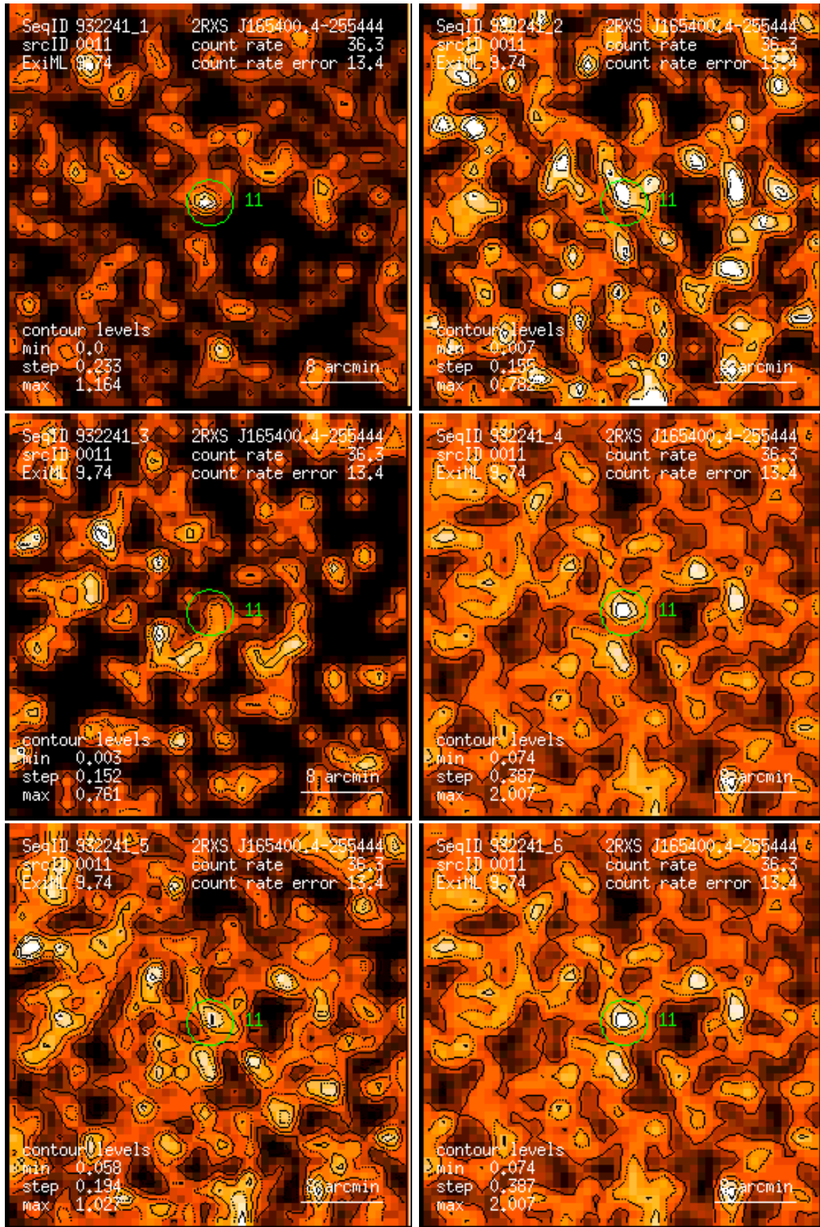
Figure 11: RASS 932241: detection 0011: band rate images, Gaussian filter: (1) PSPC channels 11 – 41, (2) 52 – 90, (3) 91 – 201, (4) 11 – 235, (5) 52 – 201, (6) 11 – 201. Broad band rates in counts/ks. Band rate contour levels in counts/ks/arcmin 2 .
