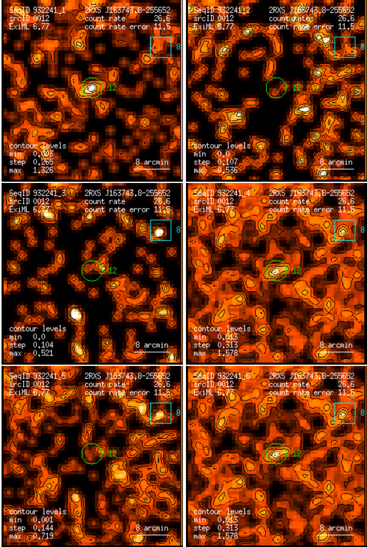
Figure 12: RASS 932241: detection 0012: band rate images, Gaussian filter: (1) PSPC channels 11 – 41, (2) 52 – 90, (3) 91 – 201, (4) 11 – 235, (5) 52 – 201, (6) 11 – 201. Broad band rates in counts/ks. Band rate contour levels in counts/ks/arcmin 2 .
