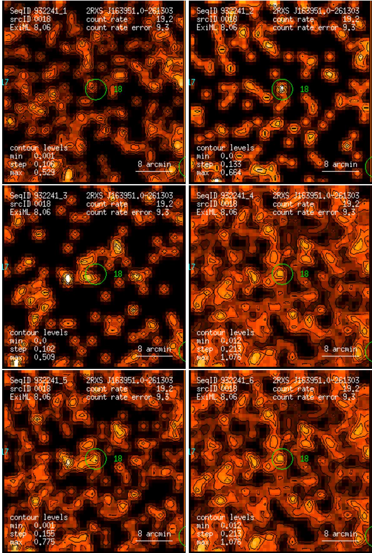
Figure 18: RASS 932241: detection 0018: band rate images, Gaussian filter: (1) PSPC channels 11 – 41, (2) 52 – 90, (3) 91 – 201, (4) 11 – 235, (5) 52 – 201, (6) 11 – 201. Broad band rates in counts/ks. Band rate contour levels in counts/ks/arcmin 2 .
