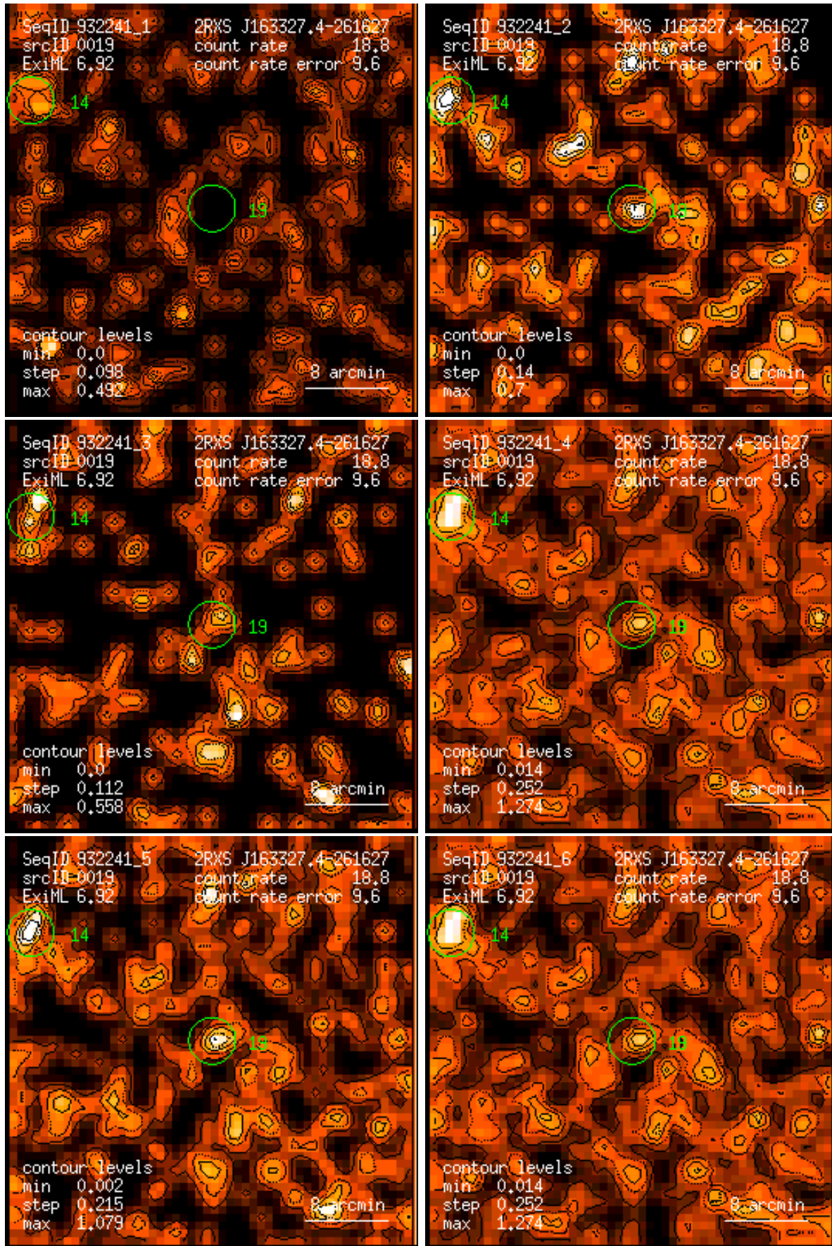
Figure 19: RASS 932241: detection 0019: band rate images, Gaussian filter: (1) PSPC channels 11 – 41, (2) 52 – 90, (3) 91 – 201, (4) 11 – 235, (5) 52 – 201, (6) 11 – 201. Broad band rates in counts/ks. Band rate contour levels in counts/ks/arcmin 2 .
