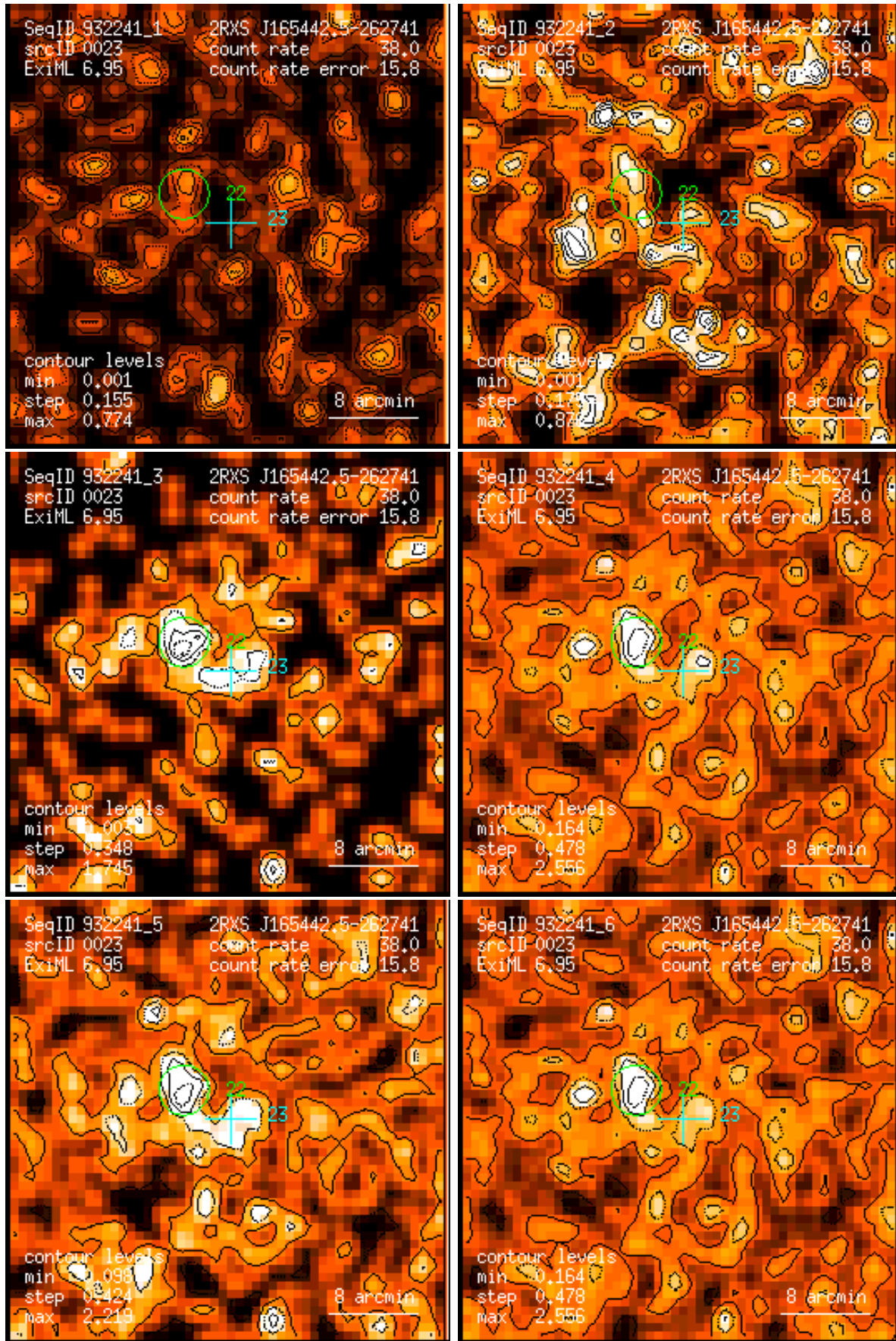
Figure 23: RASS 932241: detection 0023: band rate images, Gaussian filter: (1) PSPC channels 11 – 41, (2) 52 – 90, (3) 91 – 201, (4) 11 – 235, (5) 52 – 201, (6) 11 – 201. Broad band rates in counts/ks. Band rate contour levels in counts/ks/arcmin 2 .
