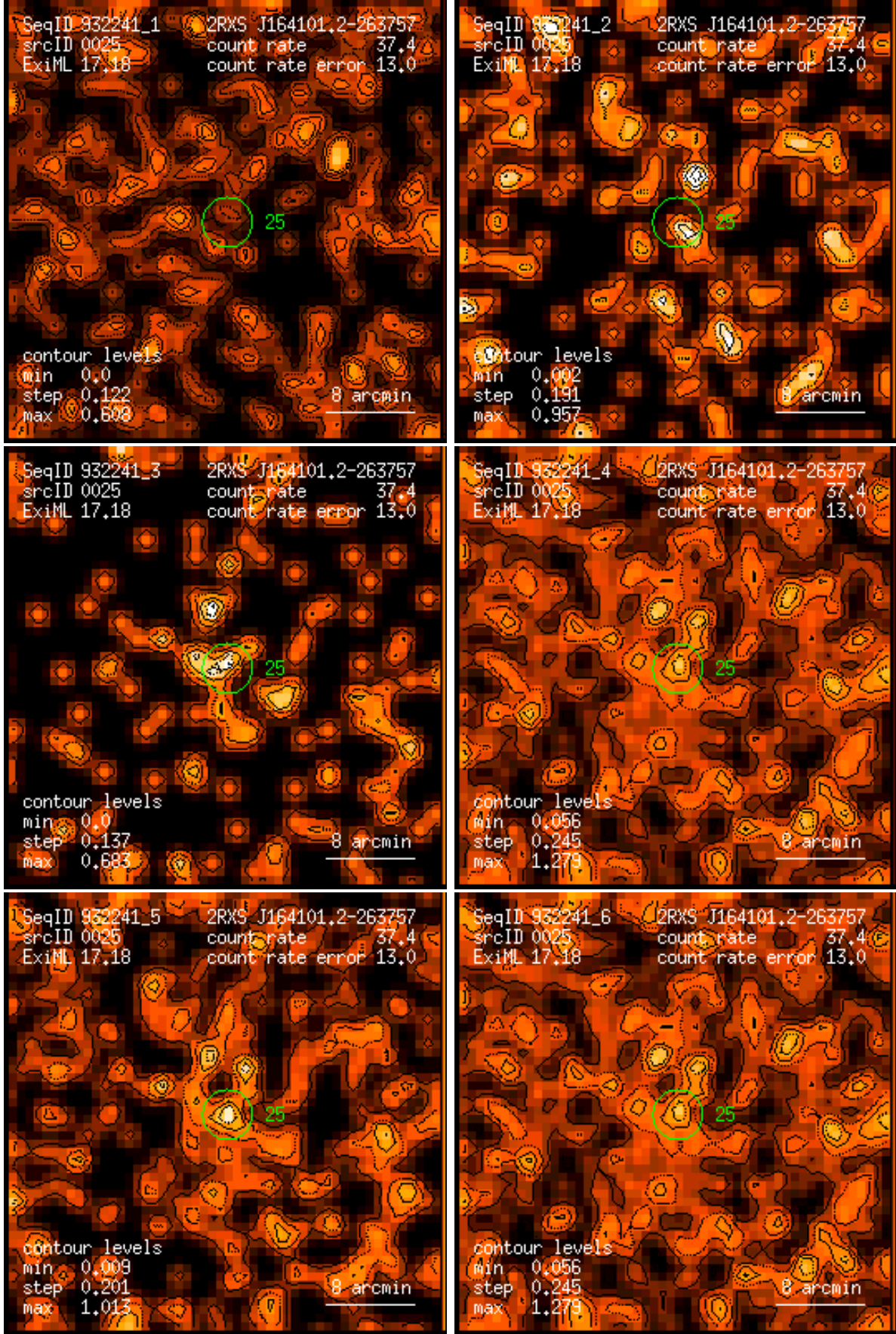
Figure 25: RASS 932241: detection 0025: band rate images, Gaussian filter: (1) PSPC channels 11 – 41, (2) 52 – 90, (3) 91 – 201, (4) 11 – 235, (5) 52 – 201, (6) 11 – 201. Broad band rates in counts/ks. Band rate contour levels in counts/ks/arcmin 2 .
