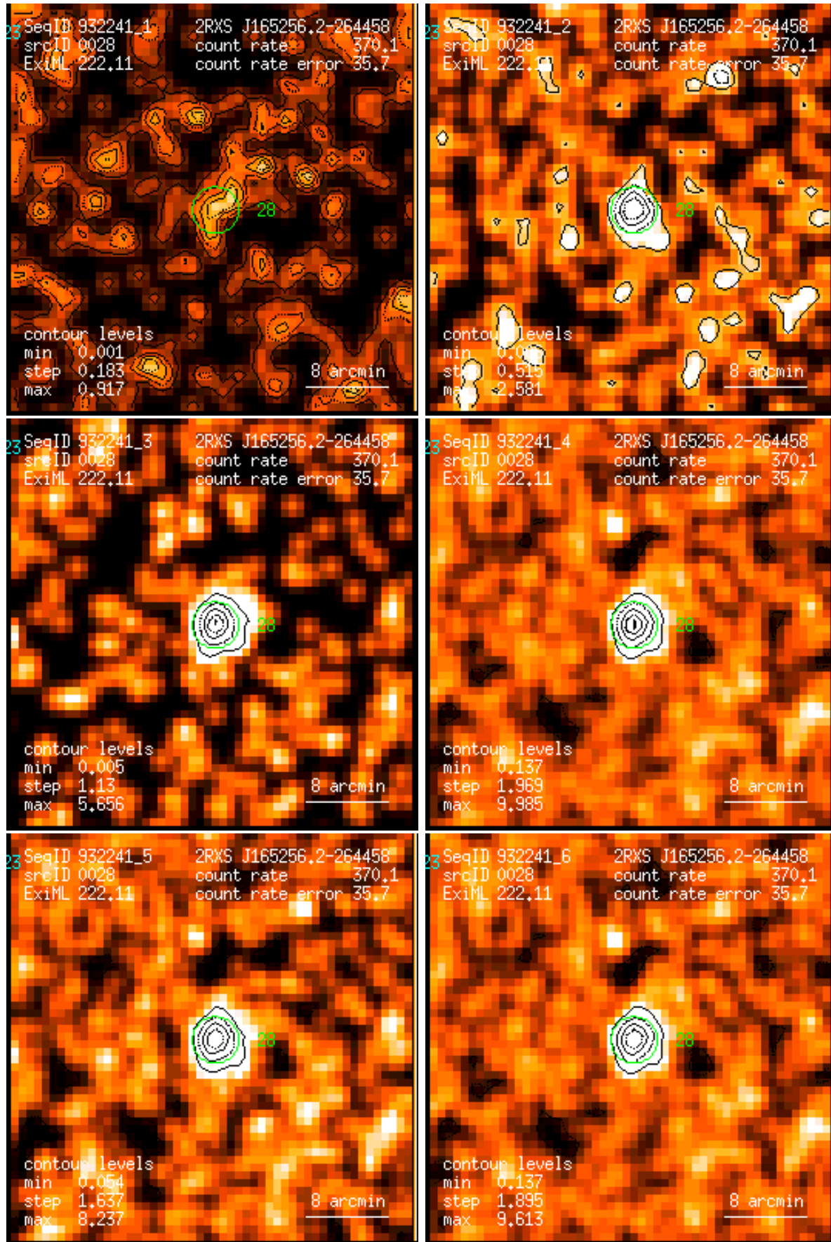
Figure 28: RASS 932241: detection 0028: band rate images, Gaussian filter: (1) PSPC channels 11 – 41, (2) 52 – 90, (3) 91 – 201, (4) 11 – 235, (5) 52 – 201, (6) 11 – 201. Broad band rates in counts/ks. Band rate contour levels in counts/ks/arcmin 2 .
