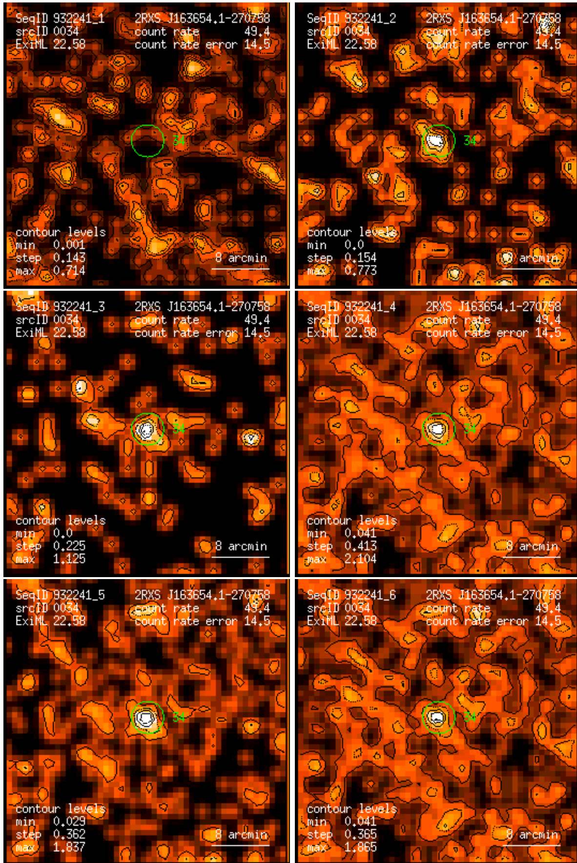
Figure 34: RASS 932241: detection 0034: band rate images, Gaussian filter: (1) PSPC channels 11 – 41, (2) 52 – 90, (3) 91 – 201, (4) 11 – 235, (5) 52 – 201, (6) 11 – 201. Broad band rates in counts/ks. Band rate contour levels in counts/ks/arcmin 2 .
