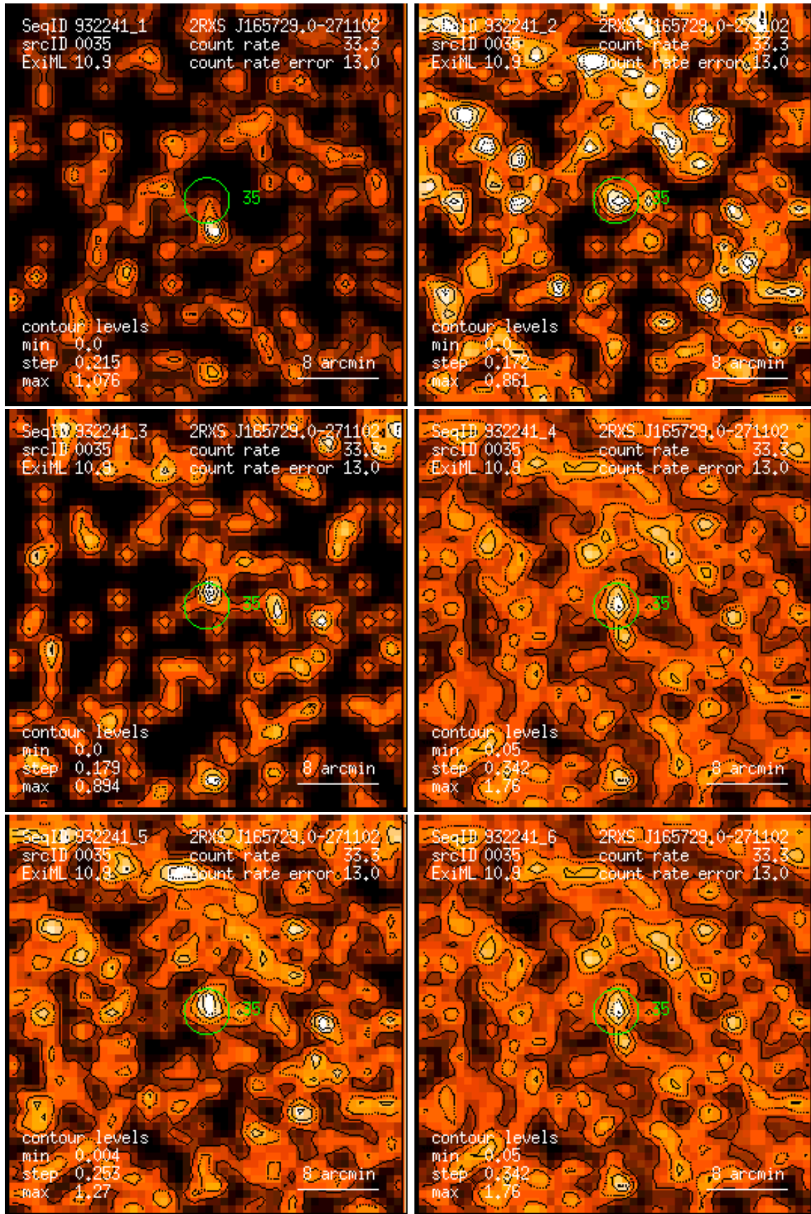
Figure 35: RASS 932241: detection 0035: band rate images, Gaussian filter: (1) PSPC channels 11 – 41, (2) 52 – 90, (3) 91 – 201, (4) 11 – 235, (5) 52 – 201, (6) 11 – 201. Broad band rates in counts/ks. Band rate contour levels in counts/ks/arcmin 2 .
