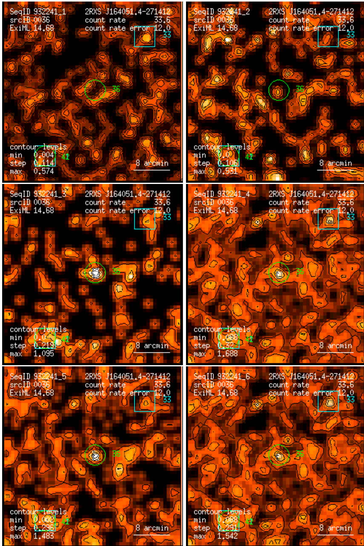
Figure 36: RASS 932241: detection 0036: band rate images, Gaussian filter: (1) PSPC channels 11 – 41, (2) 52 – 90, (3) 91 – 201, (4) 11 – 235, (5) 52 – 201, (6) 11 – 201. Broad band rates in counts/ks. Band rate contour levels in counts/ks/arcmin 2 .
