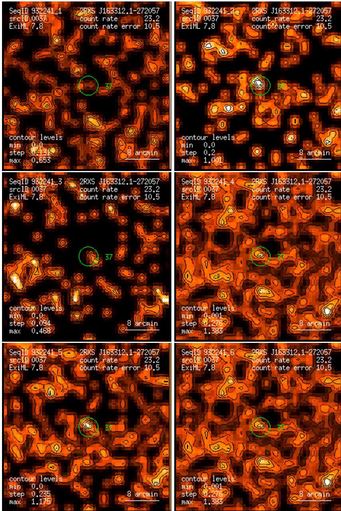
Figure 37: RASS 932241: detection 0037: band rate images, Gaussian filter: (1) PSPC channels 11 – 41, (2) 52 – 90, (3) 91 – 201, (4) 11 – 235, (5) 52 – 201, (6) 11 – 201. Broad band rates in counts/ks. Band rate contour levels in counts/ks/arcmin 2 .
