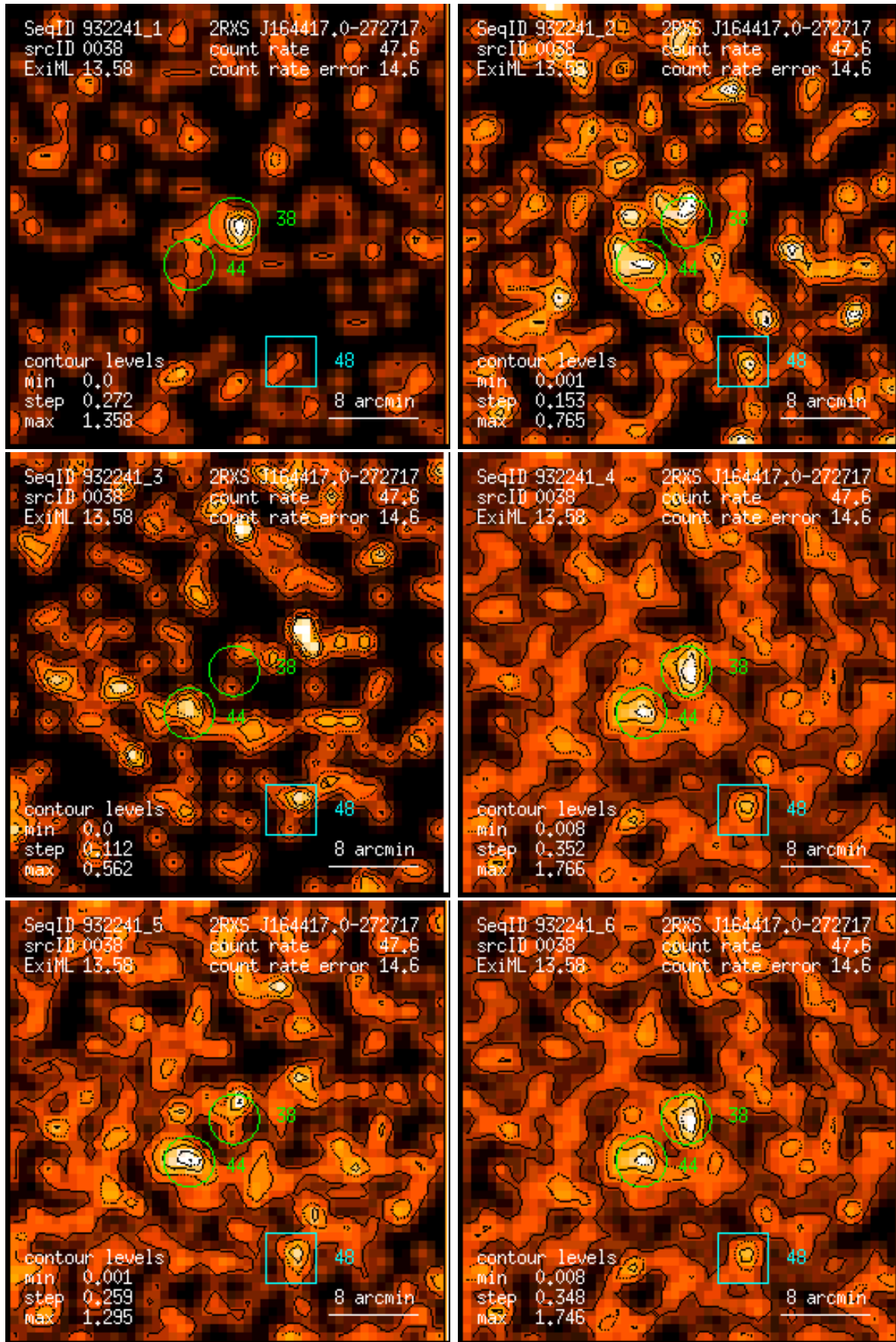
Figure 38: RASS 932241: detection 0038: band rate images, Gaussian filter: (1) PSPC channels 11 – 41, (2) 52 – 90, (3) 91 – 201, (4) 11 – 235, (5) 52 – 201, (6) 11 – 201. Broad band rates in counts/ks. Band rate contour levels in counts/ks/arcmin 2 .
