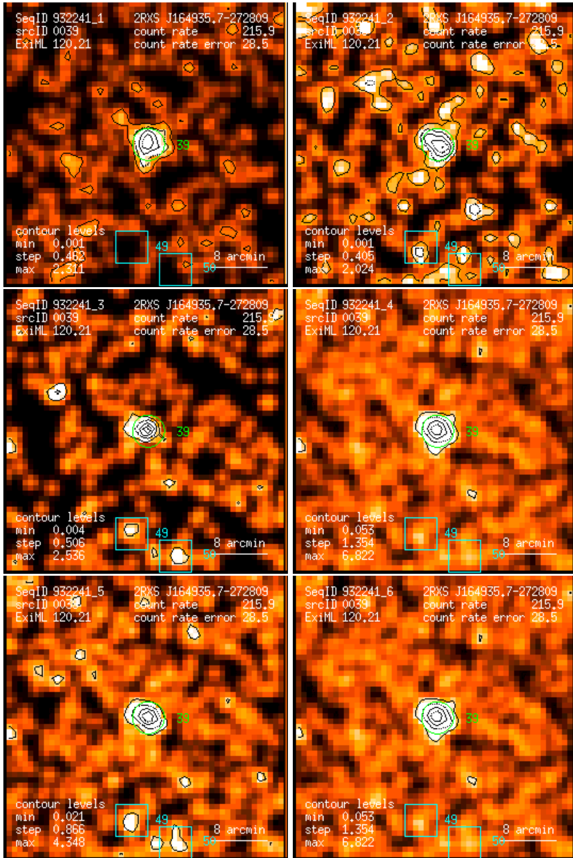
Figure 39: RASS 932241: detection 0039: band rate images, Gaussian filter: (1) PSPC channels 11 – 41, (2) 52 – 90, (3) 91 – 201, (4) 11 – 235, (5) 52 – 201, (6) 11 – 201. Broad band rates in counts/ks. Band rate contour levels in counts/ks/arcmin 2 .
