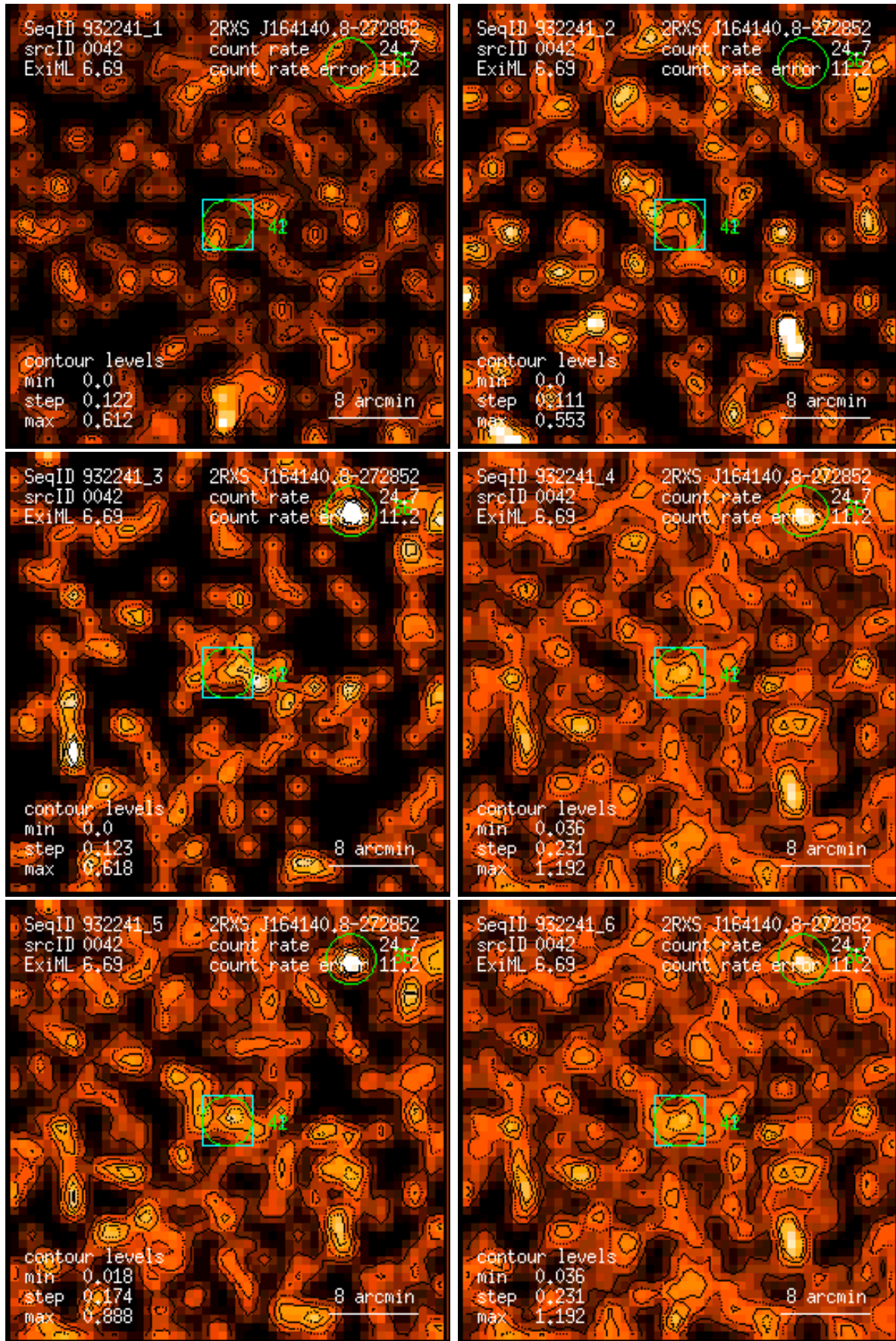
Figure 42: RASS 932241: detection 0042: band rate images, Gaussian filter: (1) PSPC channels 11 – 41, (2) 52 – 90, (3) 91 – 201, (4) 11 – 235, (5) 52 – 201, (6) 11 – 201. Broad band rates in counts/ks. Band rate contour levels in counts/ks/arcmin 2 .
