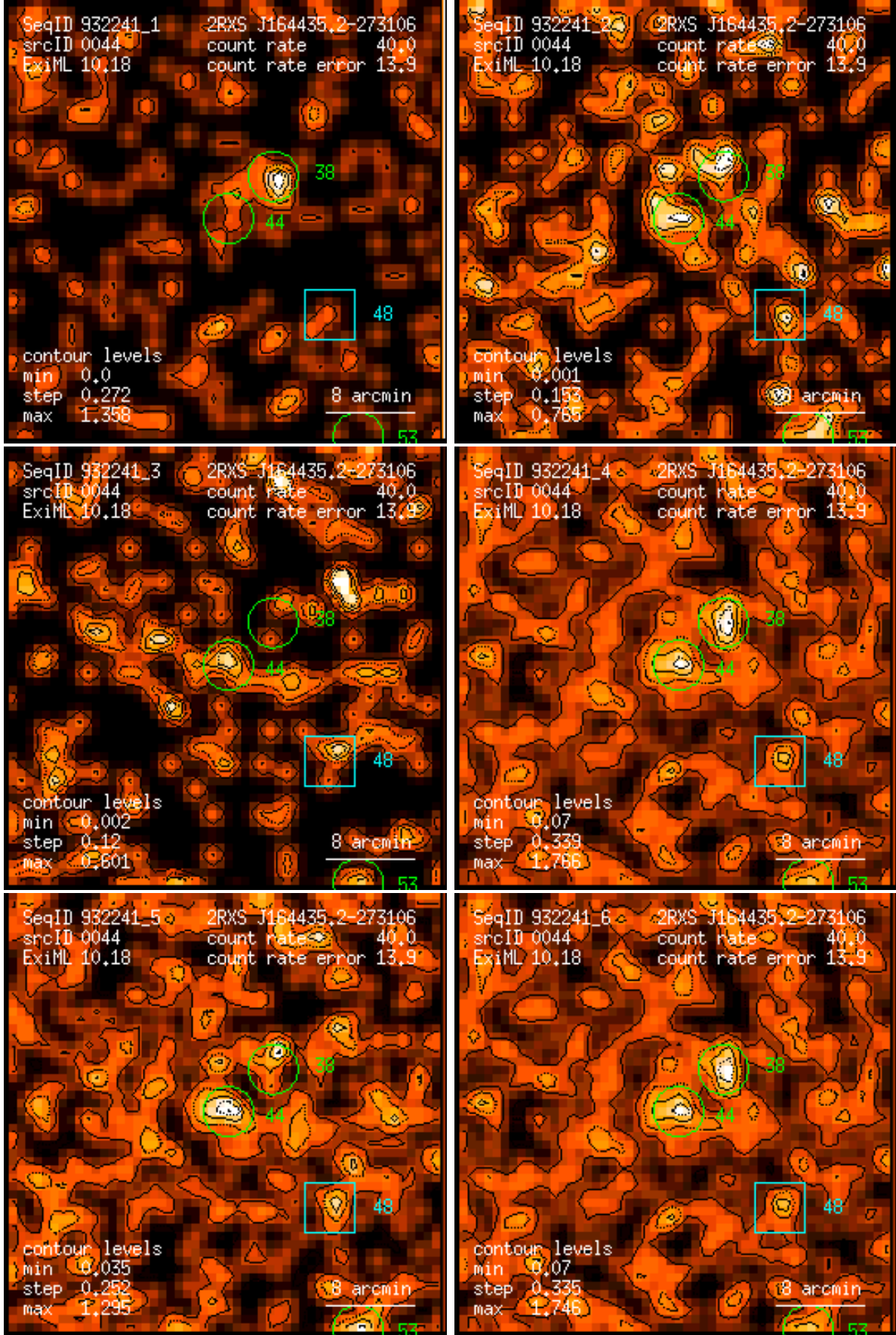
Figure 44: RASS 932241: detection 0044: band rate images, Gaussian filter: (1) PSPC channels 11 – 41, (2) 52 – 90, (3) 91 – 201, (4) 11 – 235, (5) 52 – 201, (6) 11 – 201. Broad band rates in counts/ks. Band rate contour levels in counts/ks/arcmin 2 .
