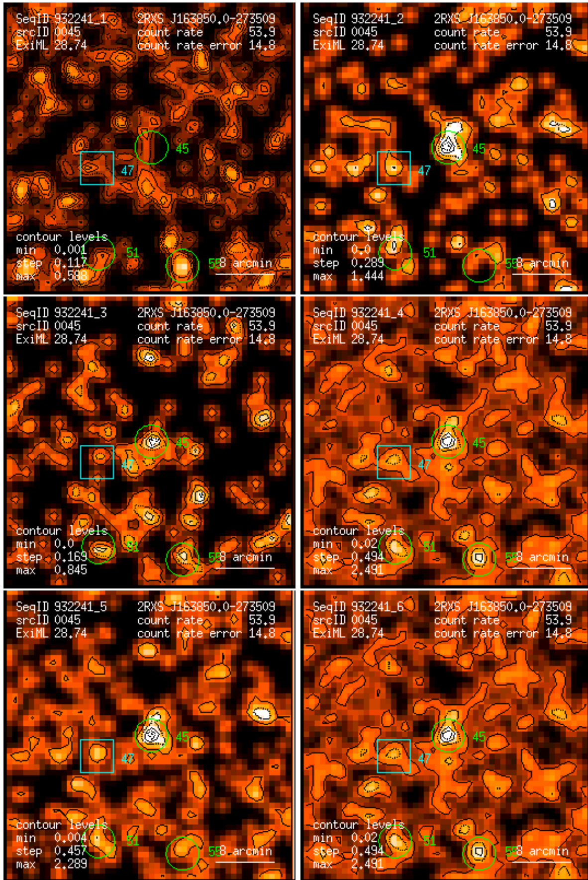
Figure 45: RASS 932241: detection 0045: band rate images, Gaussian filter: (1) PSPC channels 11 – 41, (2) 52 – 90, (3) 91 – 201, (4) 11 – 235, (5) 52 – 201, (6) 11 – 201. Broad band rates in counts/ks. Band rate contour levels in counts/ks/arcmin 2 .
