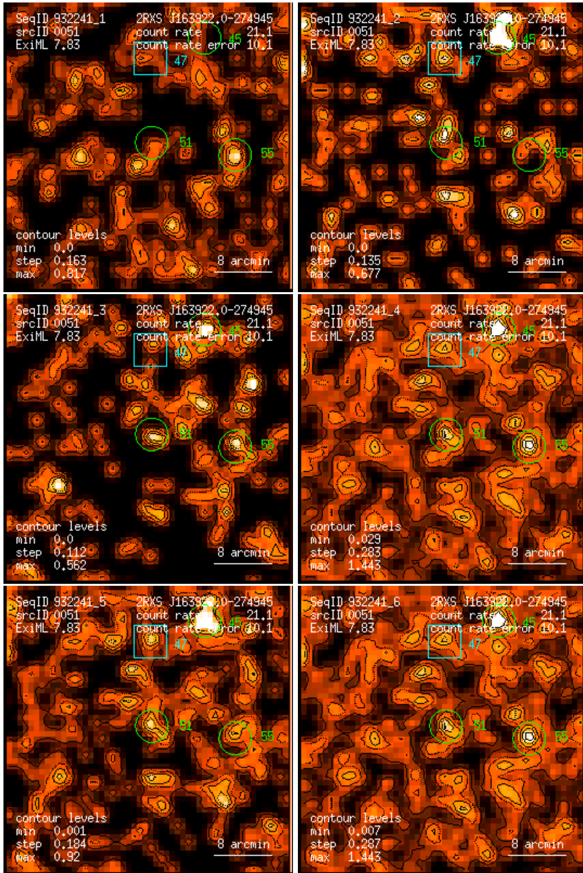
Figure 51: RASS 932241: detection 0051: band rate images, Gaussian filter: (1) PSPC channels 11 – 41, (2) 52 – 90, (3) 91 – 201, (4) 11 – 235, (5) 52 – 201, (6) 11 – 201. Broad band rates in counts/ks. Band rate contour levels in counts/ks/arcmin 2 .
