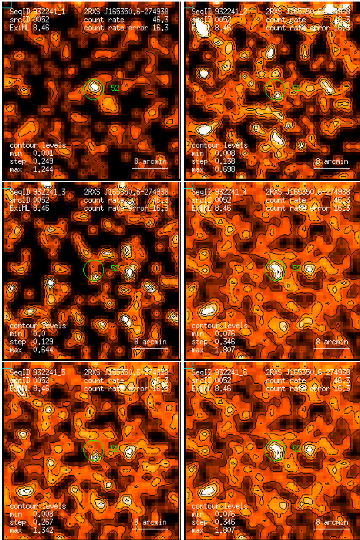
Figure 52: RASS 932241: detection 0052: band rate images, Gaussian filter: (1) PSPC channels 11 – 41, (2) 52 – 90, (3) 91 – 201, (4) 11 – 235, (5) 52 – 201, (6) 11 – 201. Broad band rates in counts/ks. Band rate contour levels in counts/ks/arcmin 2 .
